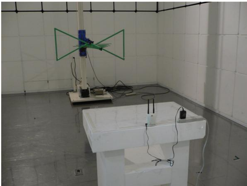
Radiated emission 2
