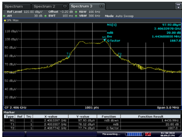
Figure 8.1-1: 20 dB Bandwidth, Low CH
