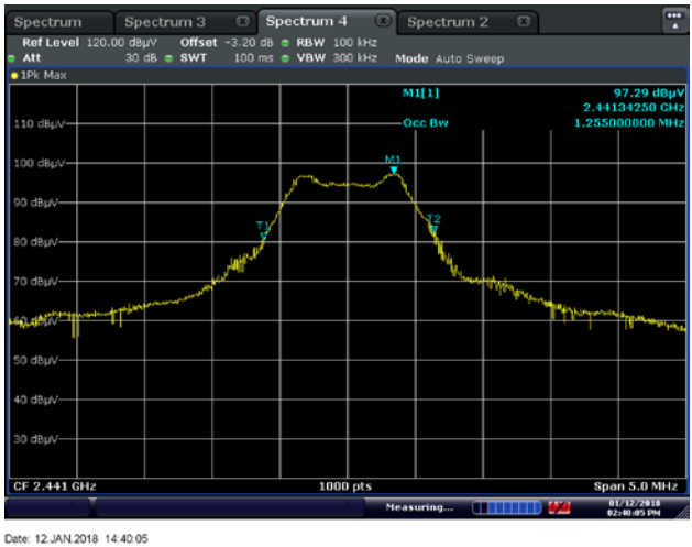
Figure 8.1-5: 99% OBW, Mid CH
