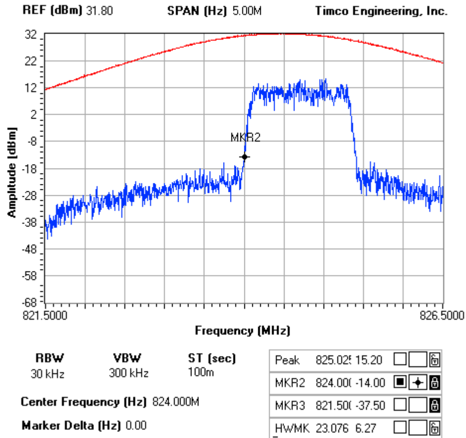
Figure 5: Band edge at 824MHz
