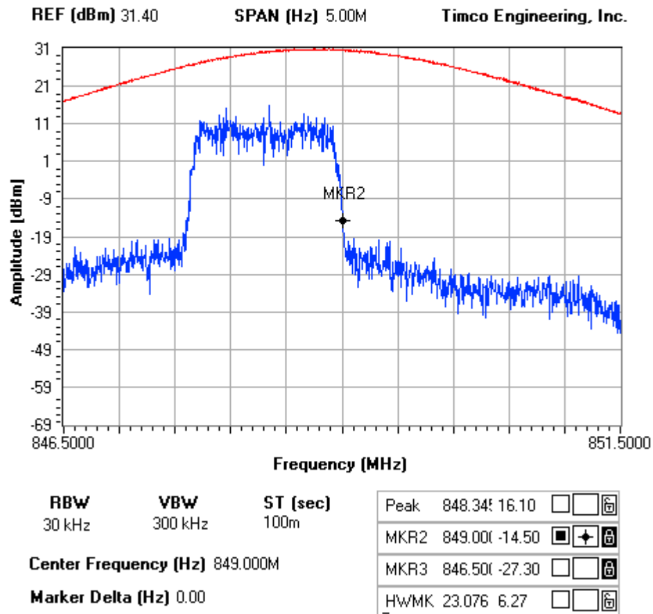
Figure 6: Band-edge at 849MHz
