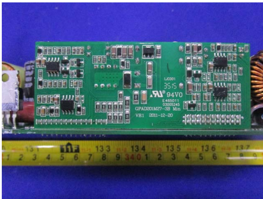
EUT –Power Sub Board Bottom View
