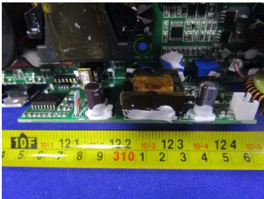
EUT –Power Sub Board Top View
