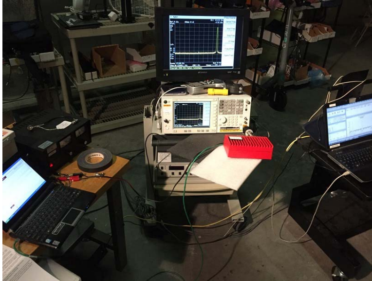
Conducted Antenna Port Measurements Power, Bandwidth, Mask, Spurious
