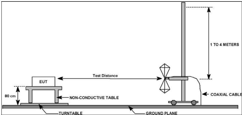
Field Strength of Radiated Emissions Test Setup
