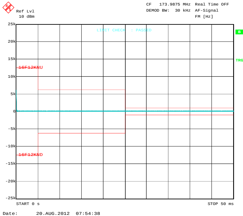
GRAPH 33: Transient behaviour, carrier frequency as a function of time, CH 1, switch ON
