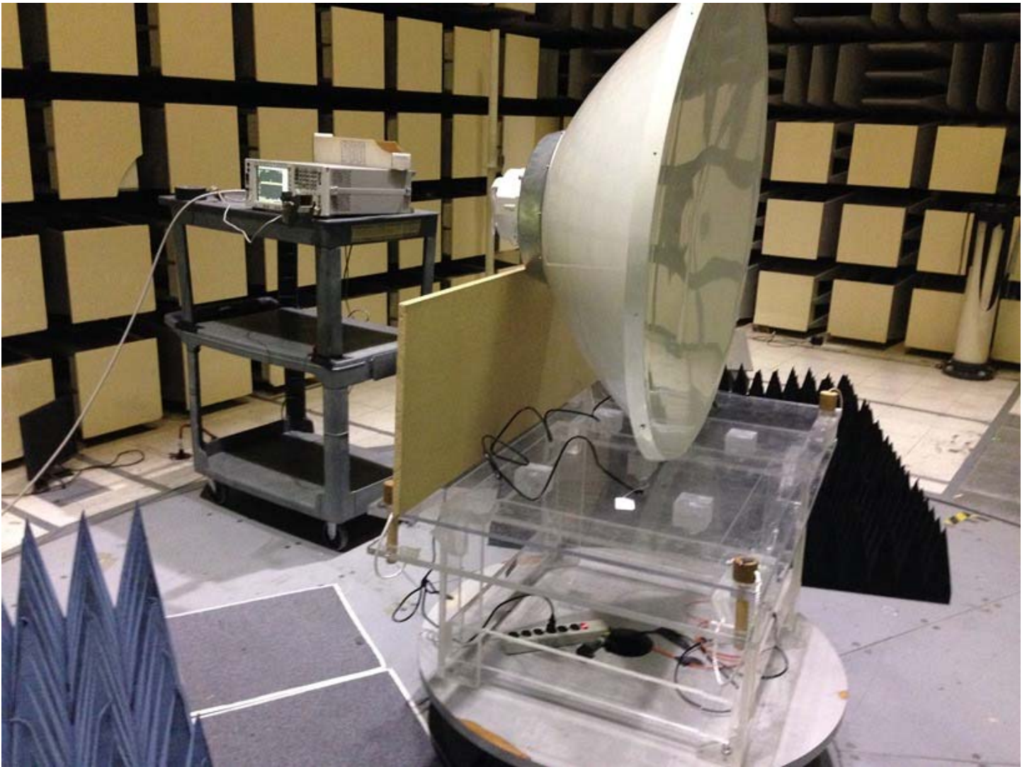
Radiated Emissions: 18 to 26.5 GHz, Front
