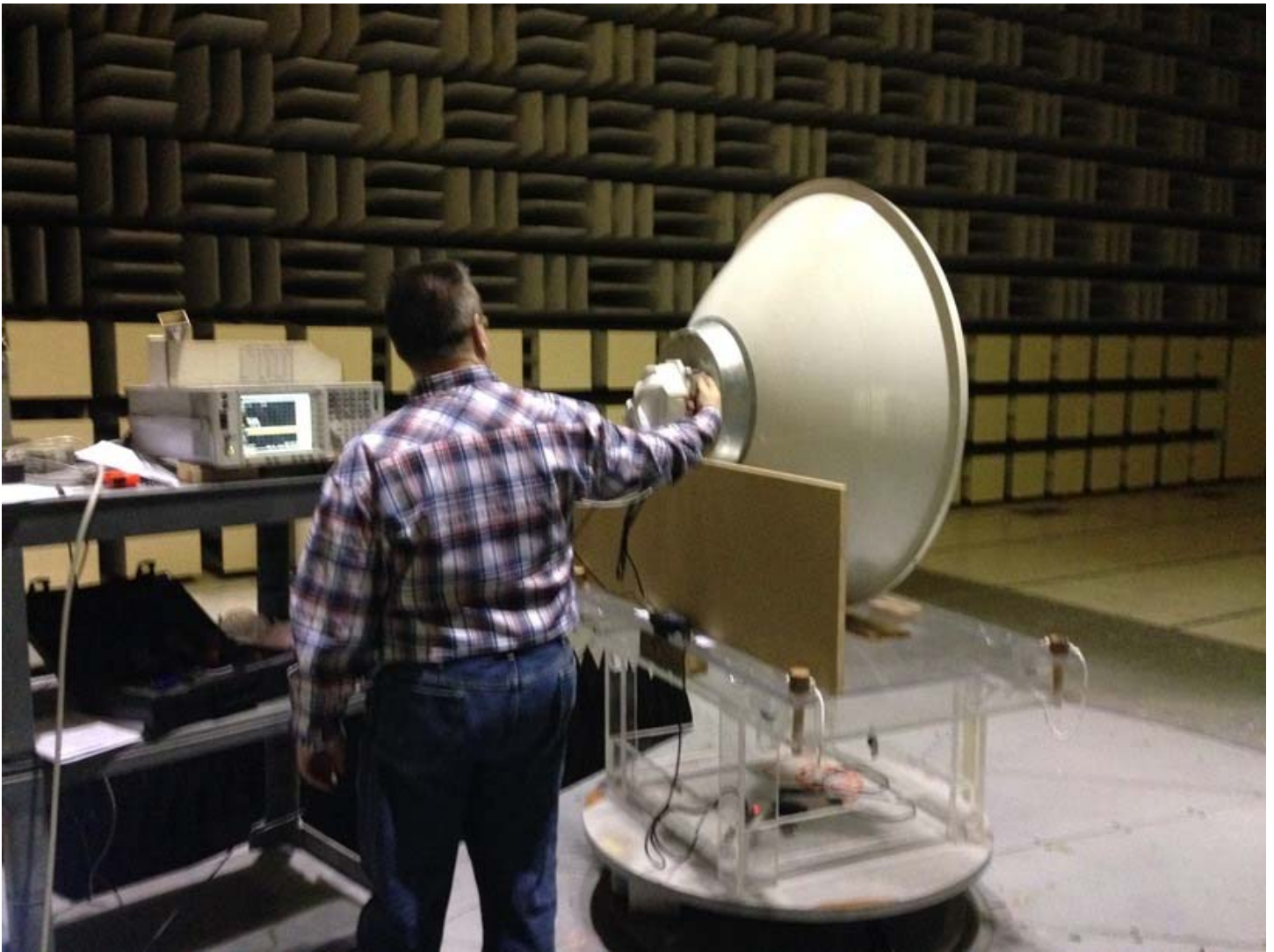
Radiated Emissions: 26.5 to 100 GHz, Front
