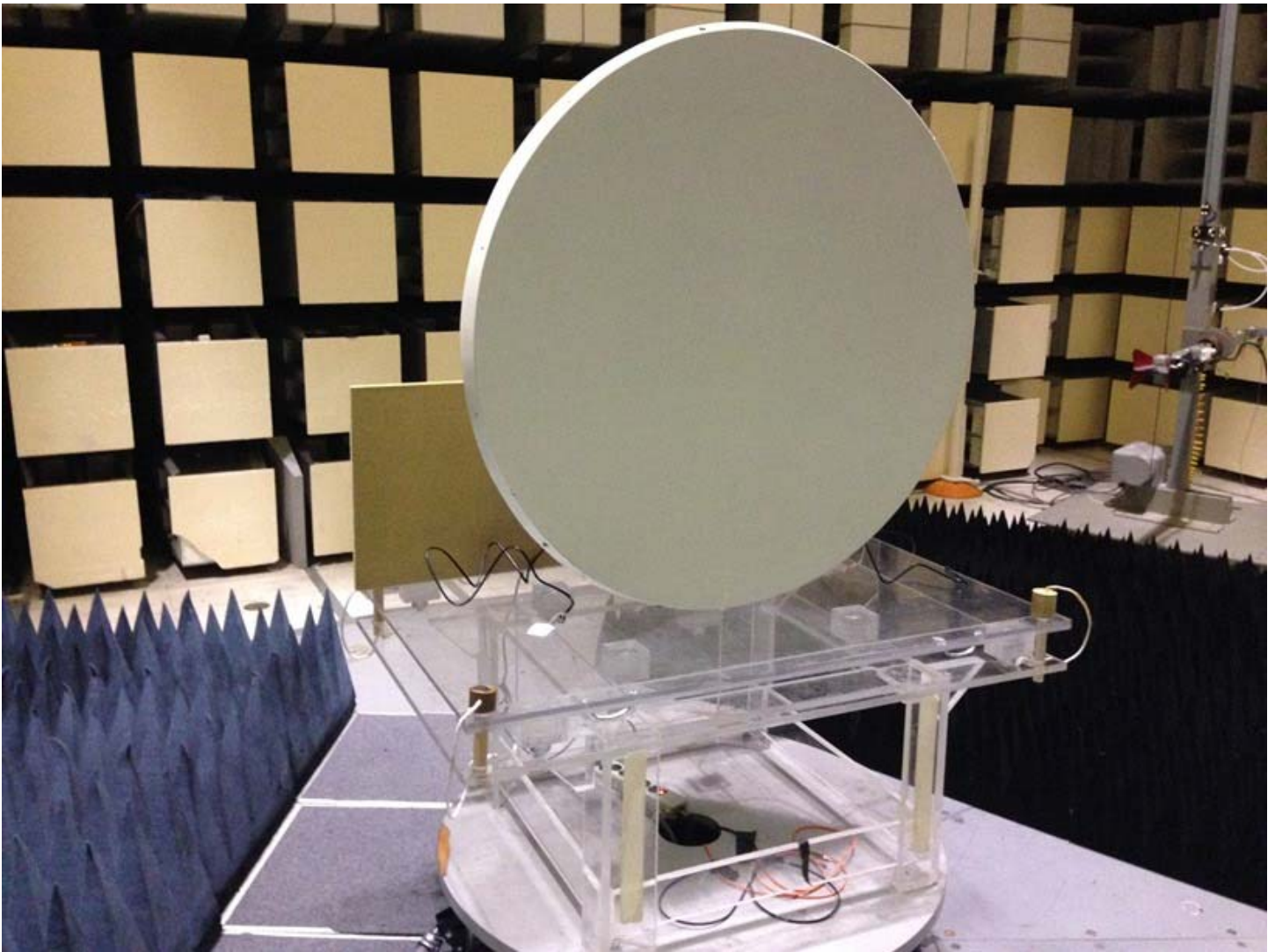
Radiated Emissions: 30 MHz to 18 GHz, Front
