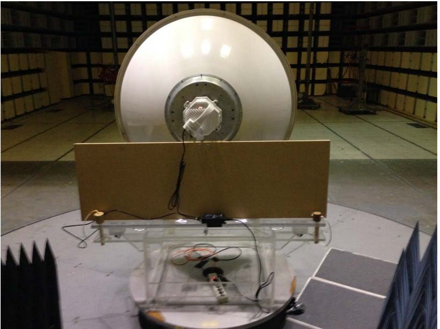
Radiated Emissions: 30 MHz to 18 GHz, Back
