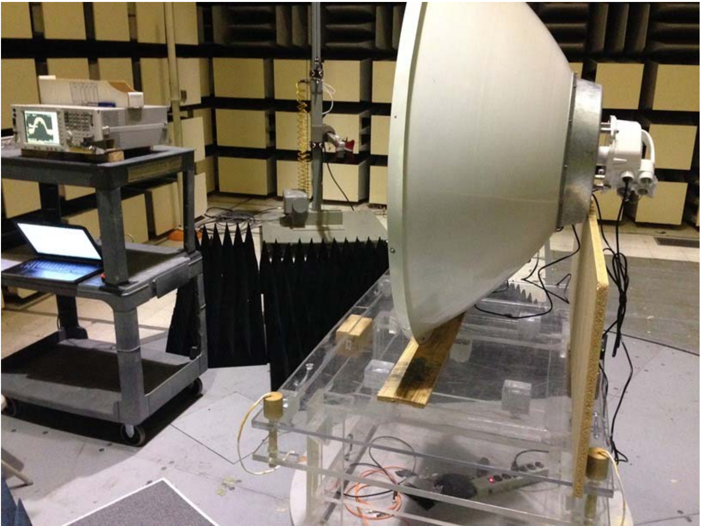
Radiated Emissions: Fundamental Field Strength
