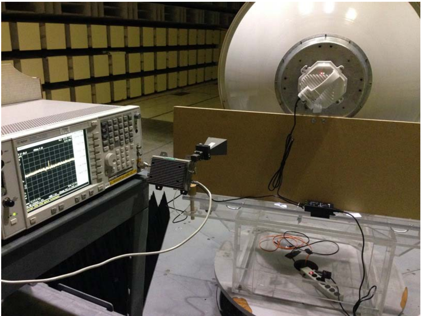
Radiated Emissions: 18 to 26.5 GHz, Back
