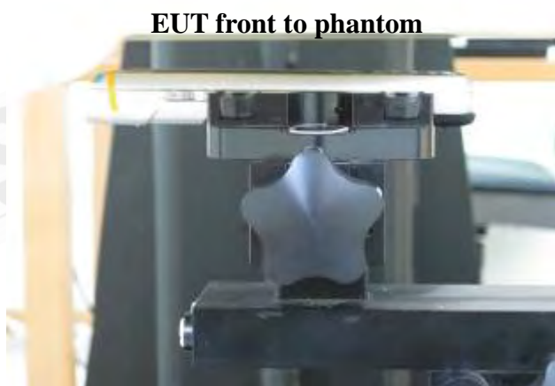
Fig.7 Body worn- EUT front to flat phantom and distance between flat phantom and mobile phone is 1.5 cm
