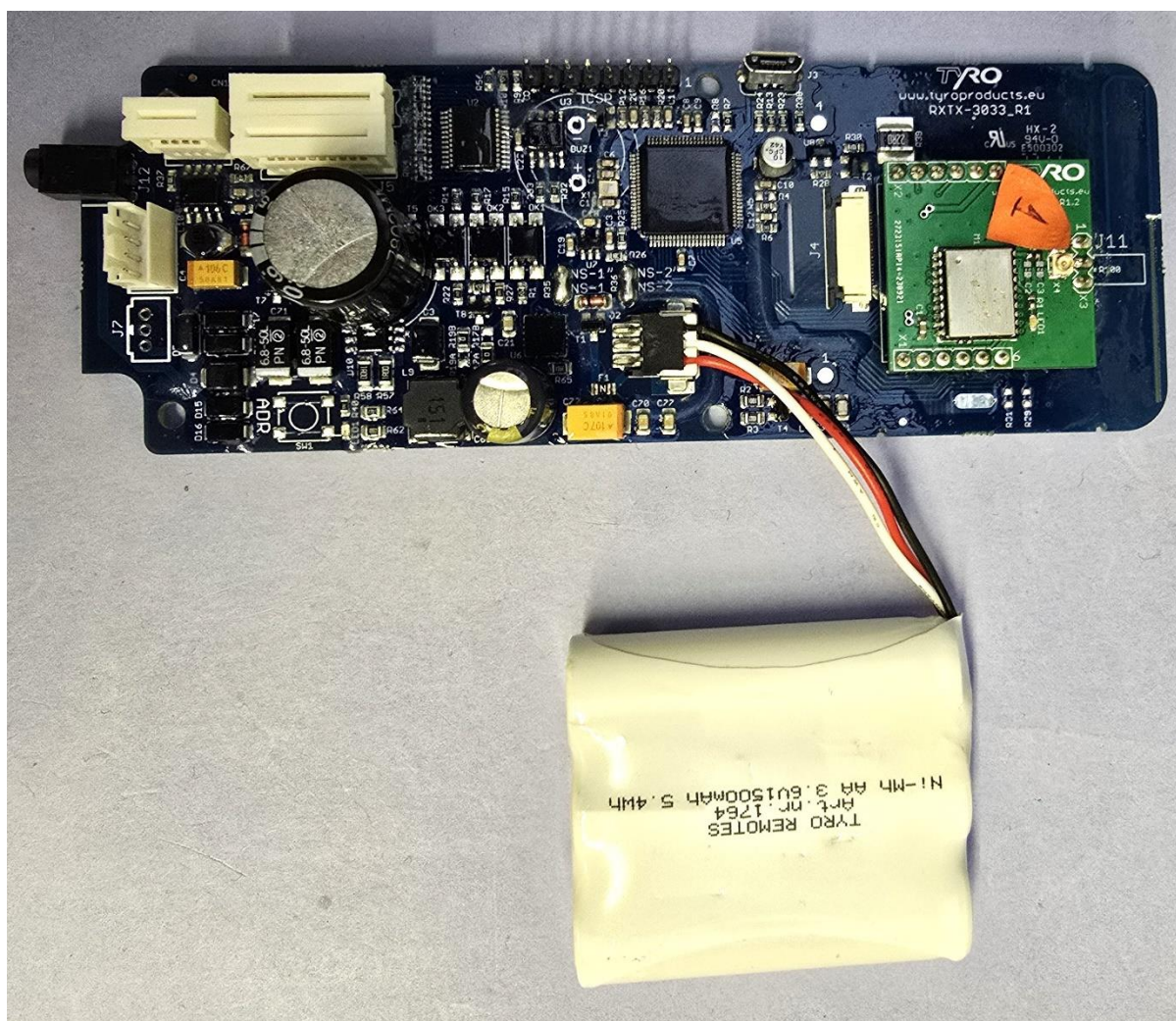
Test fixture top side
