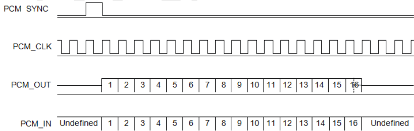
Figure 5: Short Frame Sync (Shown with 16-bit Sample)
