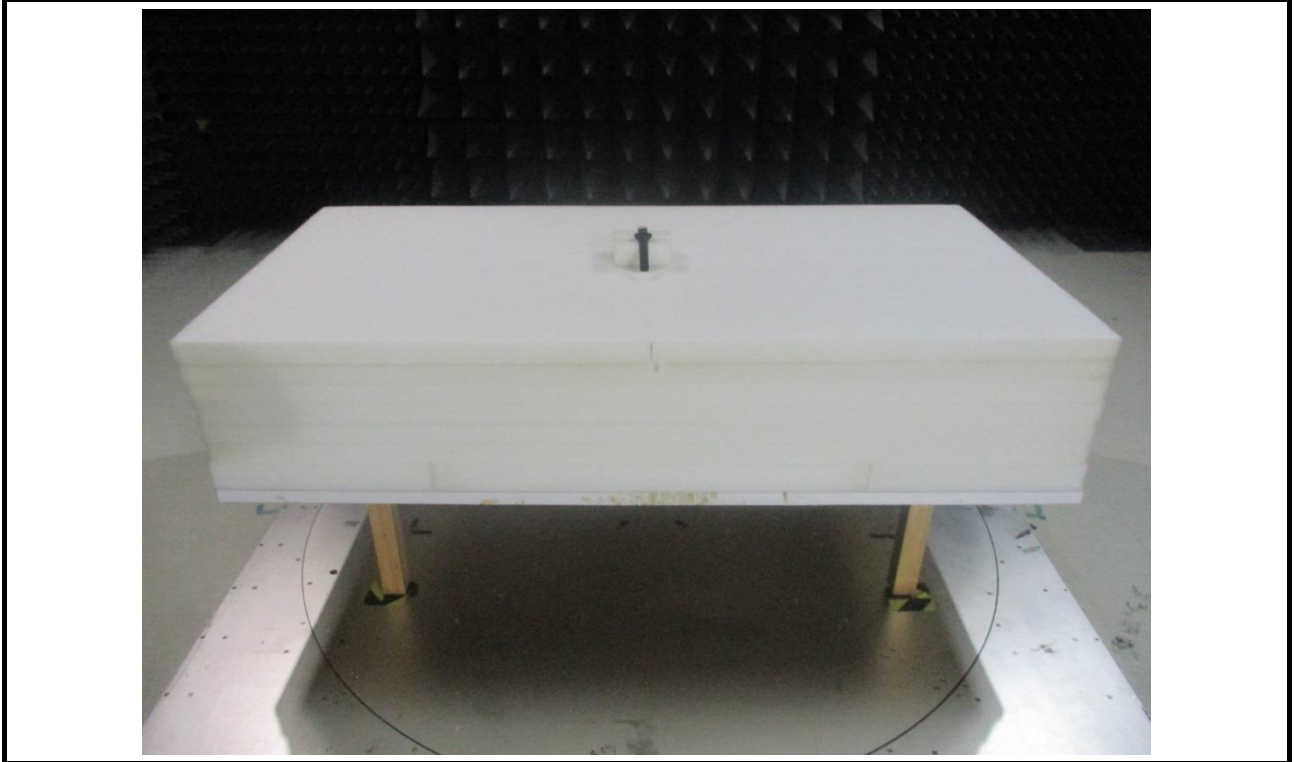
Radiated Emission Below 1GHz Test (vibrated version)
