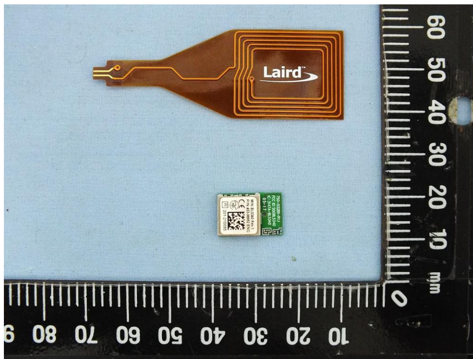
Internal Antenna
