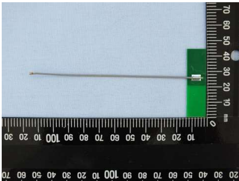
Antenna: NanoBlue
