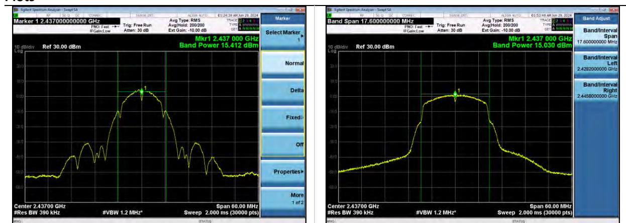
802.11b | Channel 6 | 1 Mbps
