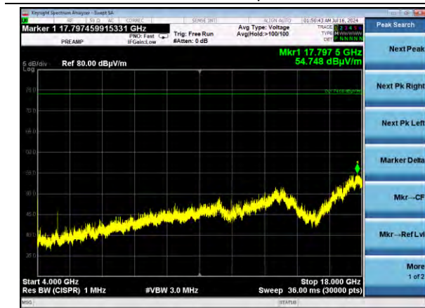
802.11b | Channel 6 | 1 Mbps | X Plane 4000-18000 MHz | Horizontal
