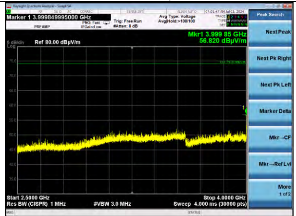
802.11b | Channel 1 | MCS11 2500-4000 MHz | Vertical
