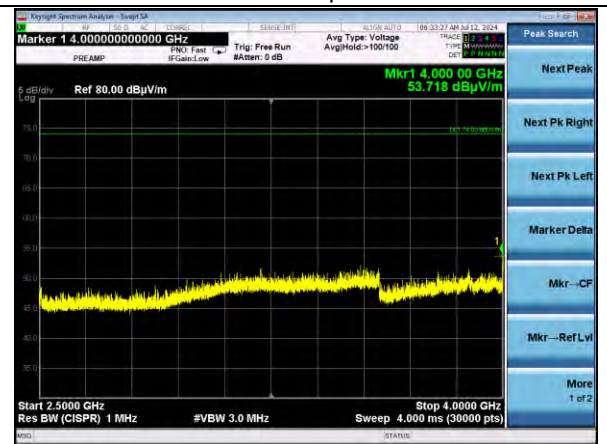
802.11b | Channel 1 | 1 Mbps | X Plane 2500-4000 MHz | Horizontal
