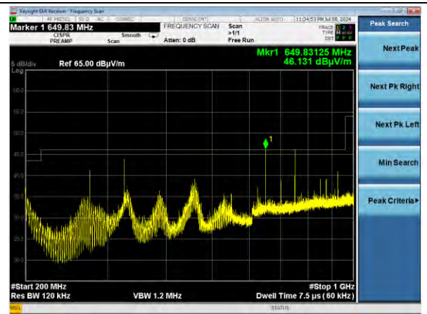
802.11b | Channel 1 | 1 Mbps | Z Plane 200-1000 MHz | Horizontal
