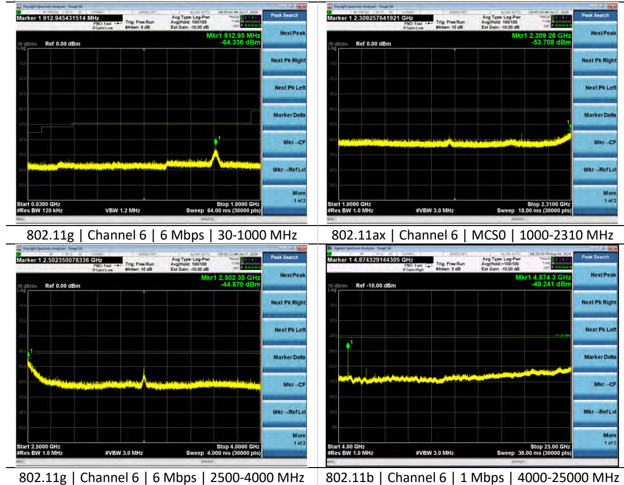
802.11g | Channel 6 | 6 Mbps | 30-1000 MHz 802.11ax | Channel 6 | MCS0 | 1000-2310 MHz 802.11g | Channel 6 | 6 Mbps | 2500-4000 MHz 802.11b | Channel 6 | 1 Mbps | 4000-25000 MHz
