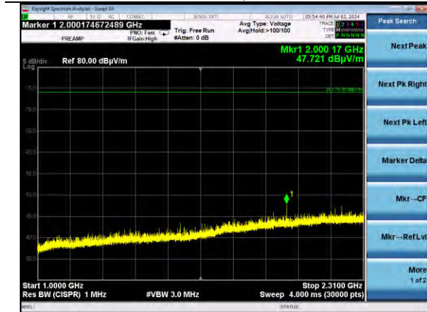
802.11b | Channel 11 | 1Mbps | 1000-2310 MHz | Vertical
