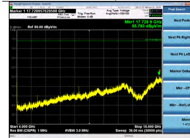
802.11b | Channel 6 | 1 Mbps 4000-18000 MHz | Vertical
