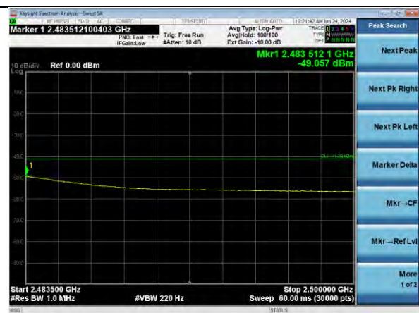
802.11ax | Channel 11 | MCS0 | Average
