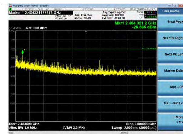
802.11ax | Channel 11 | MCS0 | Peak
