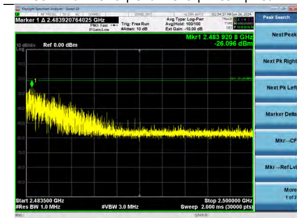
802.11ax RU52 | Channel 11 | MCS7 | Peak
