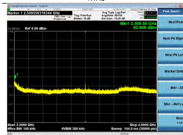
802.11ax RU26 | Channel 6 | MCS0 | 2500-4000 MHz
