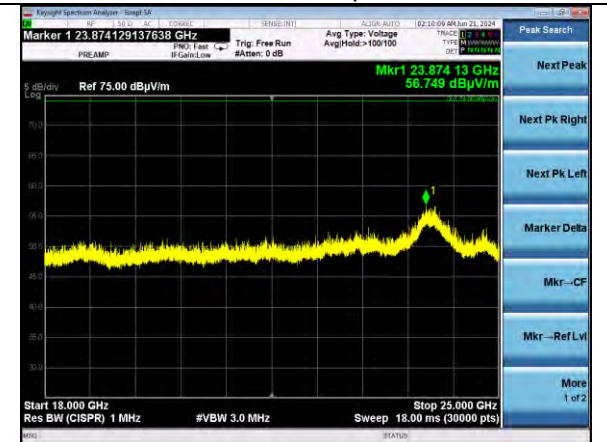
802.11b | Channel 11 | 1 Mbps 18000-25000 MHz | Horizontal
