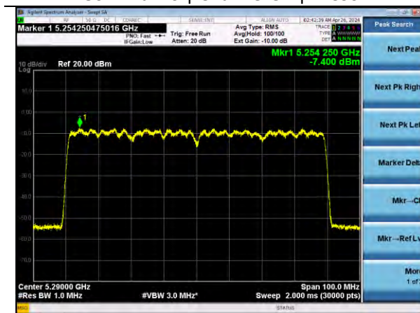
802.11ax80 | Channel 58 | MCS11
