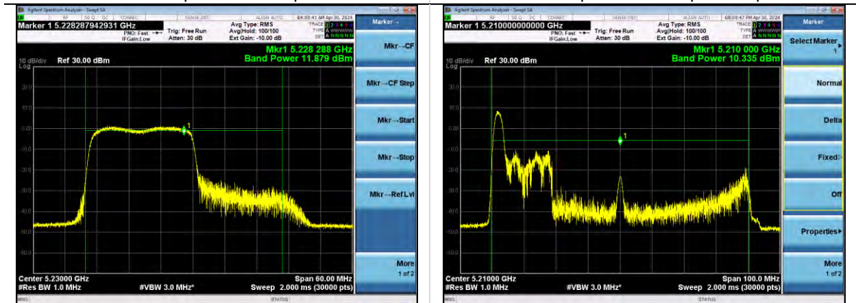
802.11ax40 | Channel 46 | MCS0 | RU 242
