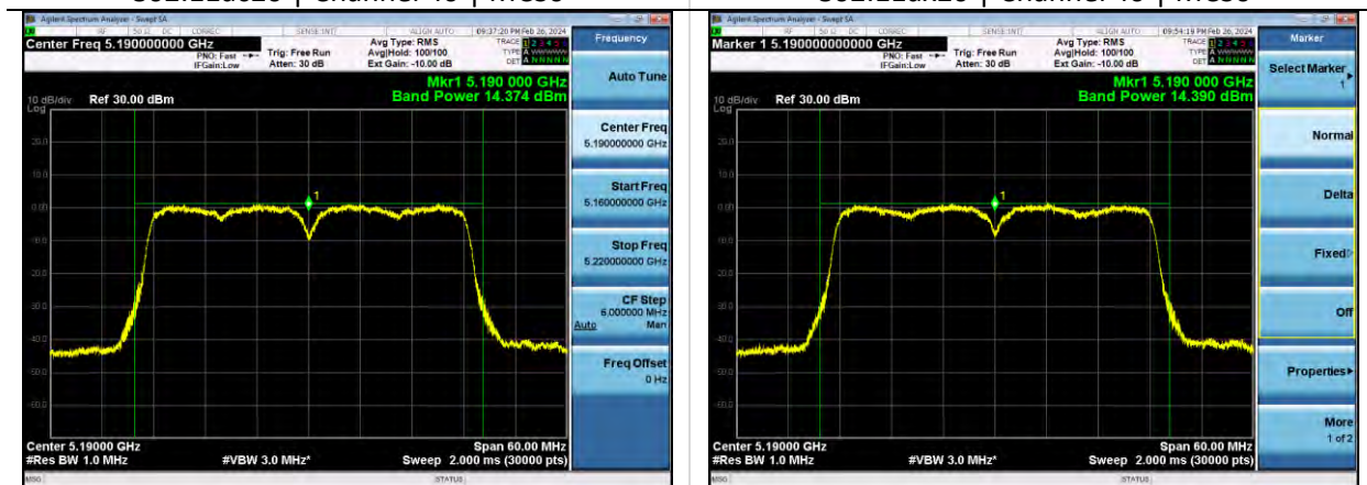
802.11n40 | Channel 38 | MCS7
