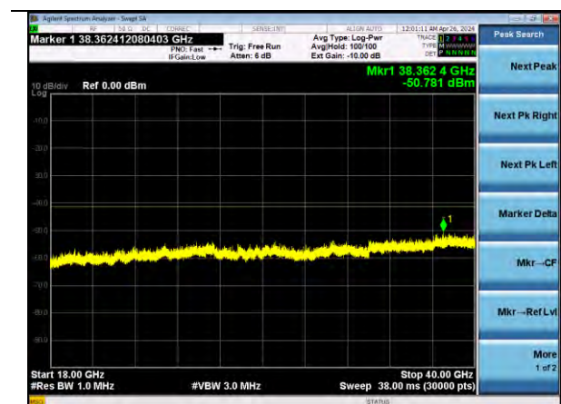
802.11a | Channel 36 | 6 Mbps | 18000-40000 MHz
