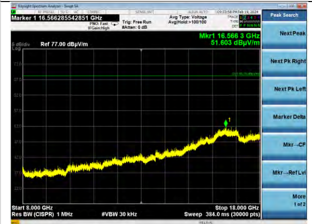
802.11a | Channel 36 | 6 Mbps | X Plane 8000-18000 MHz | Vertical
