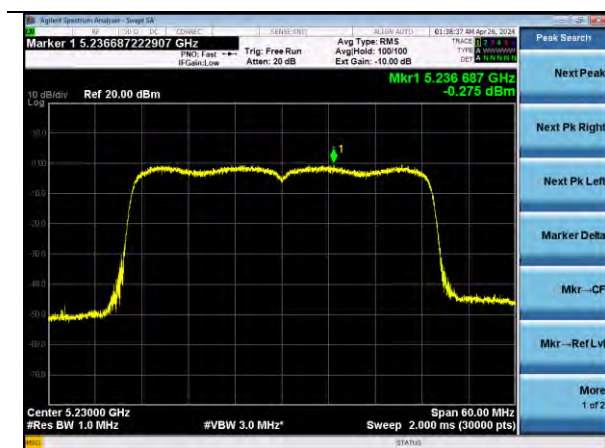
802.11ax40 | Channel 46 | MCS0
