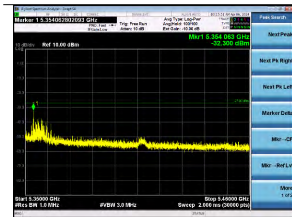
802.11ax20 | Channel 64 | MCS0 | RU52 | Peak
