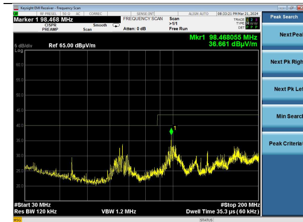
Channel 19 | 1 Mbps 30-200 MHz | Horizontal
