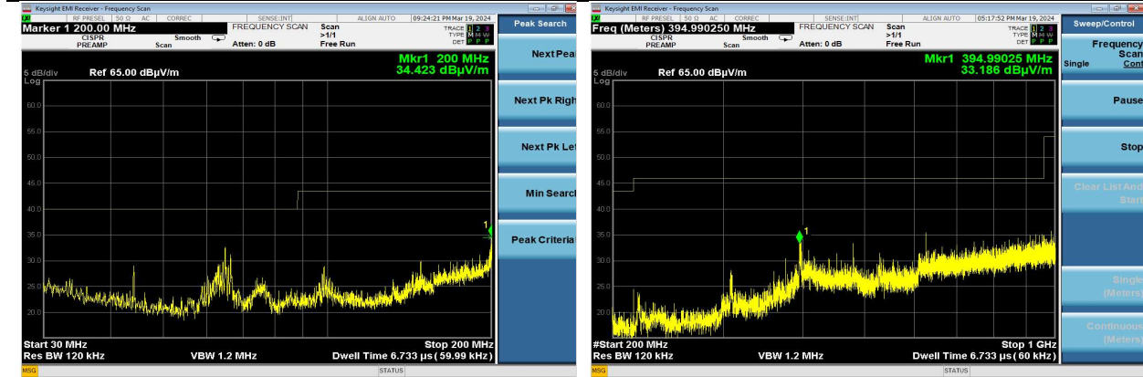
Channel 39 | Basic Rate | Single 30-200 MHz | Horizontal
