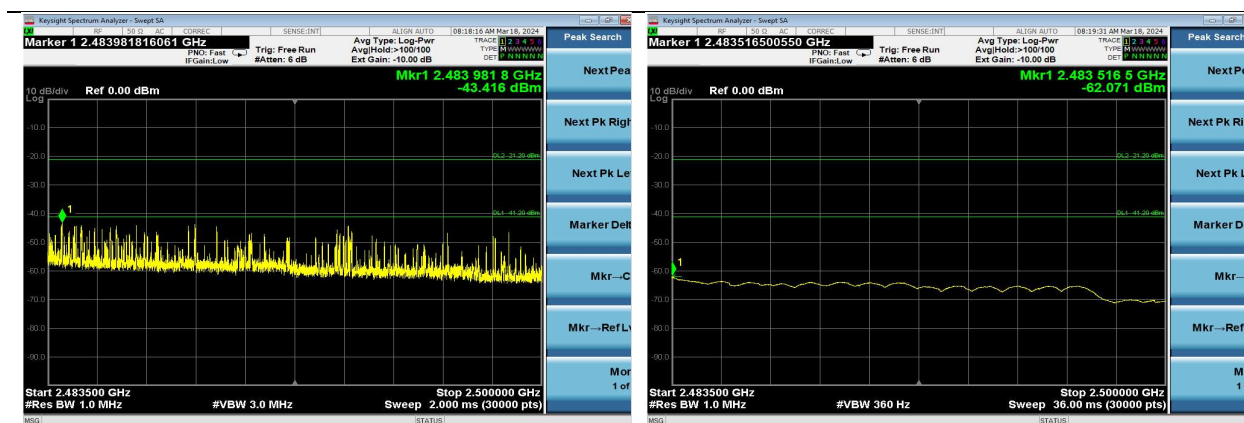
Hopping | DH5 | 2483.5-2500 MHz | Peak
