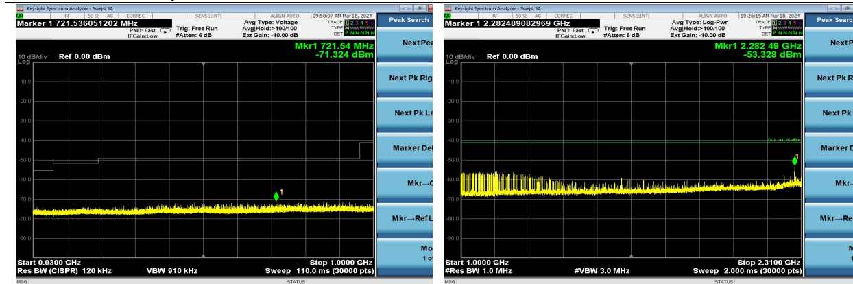
Channel 0 | DH5 | 30-1000 MHz
