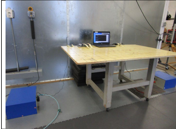
AC Mains Conducted Emissions
