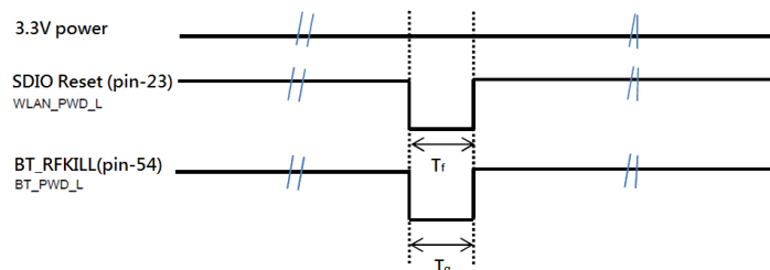
Figure 2: Reset Timing
