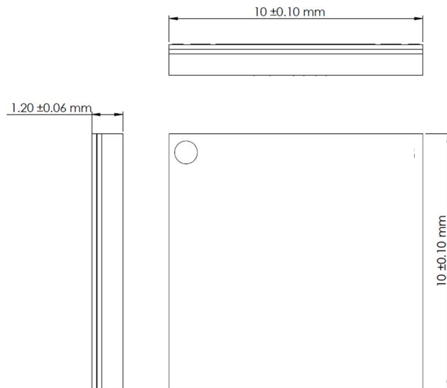
Figure 9: Base SiP module mechanical dimensions
