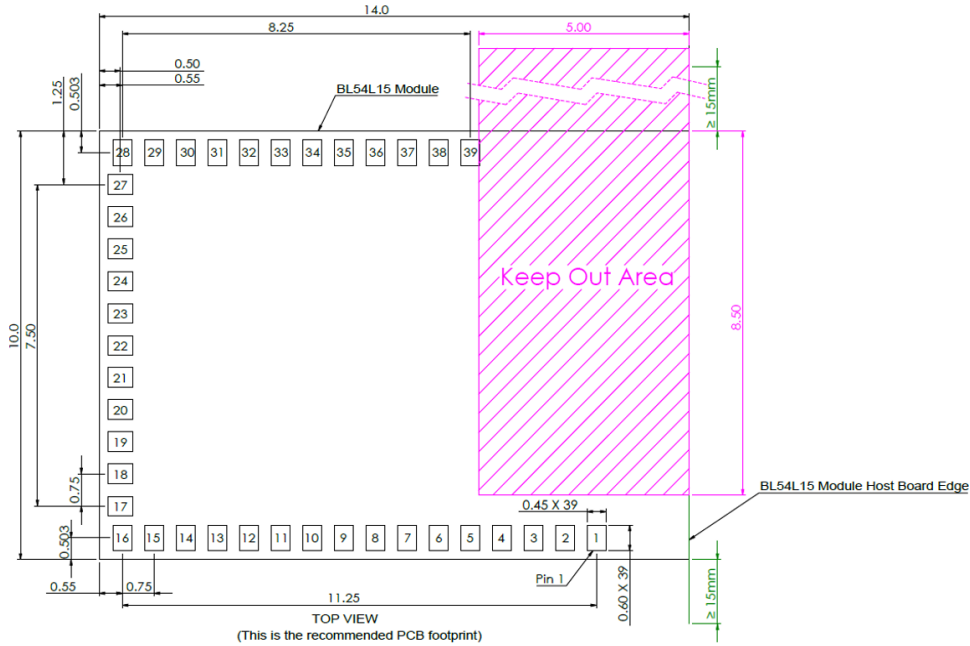
Figure 9: Land pattern and Keep-out for the 453-00001
