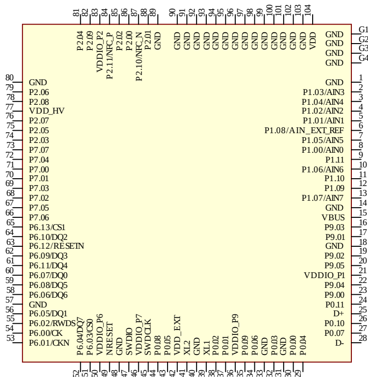
Figure 2: Top view - Schematic symbol for 453-00197 BL54H20 Multi-Core/Protocol-Bluetooth +802.15.4+NFC Module (Nordic nRF54H20) - Integrated Antenna (Ignion chip antenna) or MHF4 RF connector variant 453-00198
