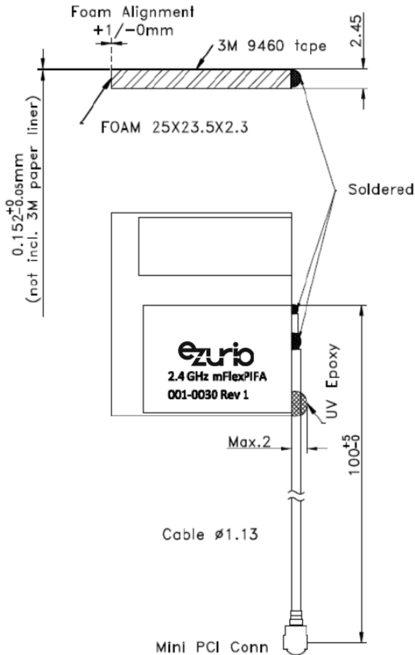
Figure 1: Physical dimensions
