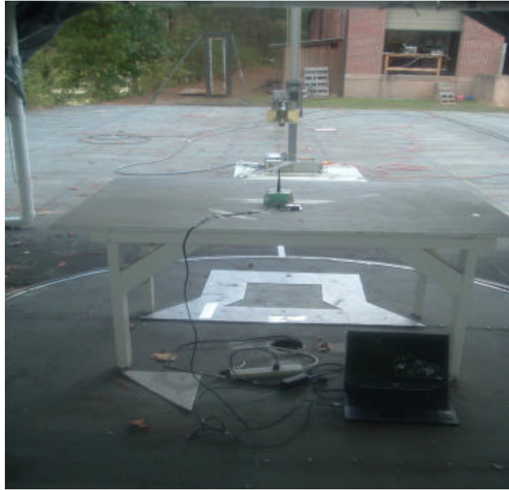
Photo 2. Test Setup above 1 GHz testing
