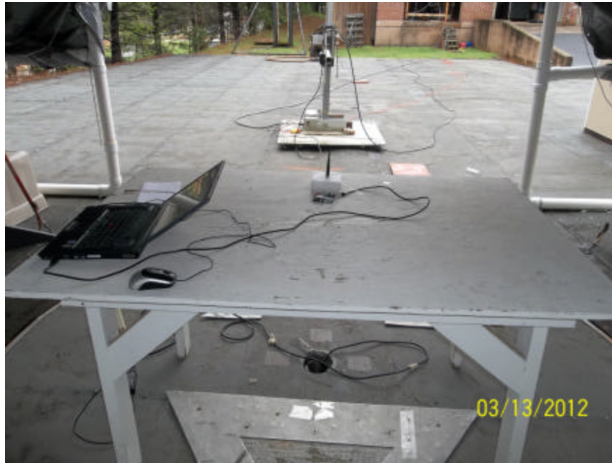
Photo 4. Test Setup 9 kHz to 30 MHz testing.
