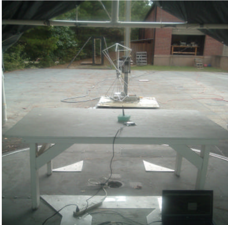
Photo 3. Test Setup 30 MHz – 200 MHz testing
