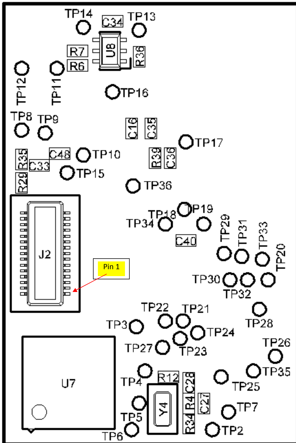
Figure 3. VN400 PC Board Bottom View Showing J2, Pin 1 Location
