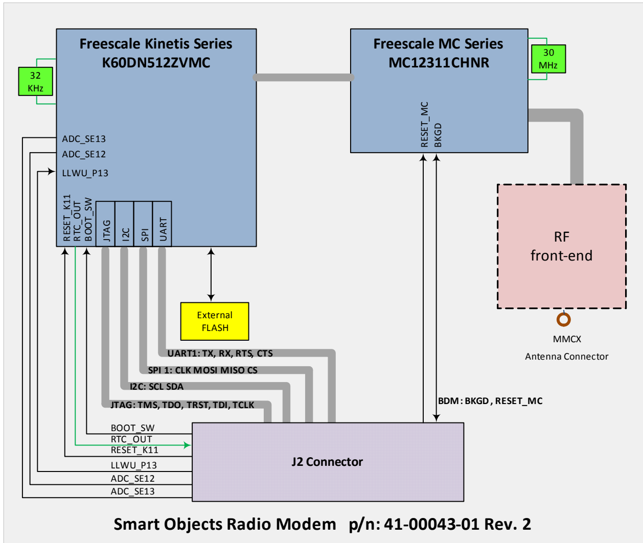
Figure 1. VN400 Functional Block Diagram
