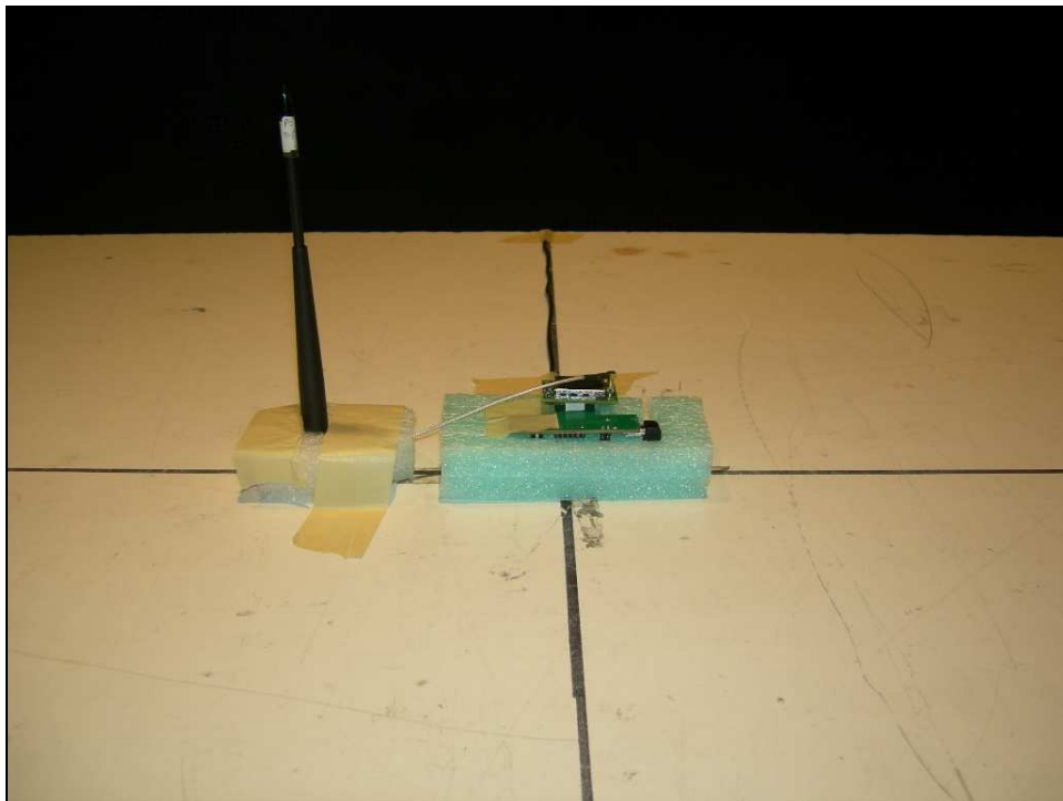
Figure 1: Radiated Emissions Test Setup – XPOS
