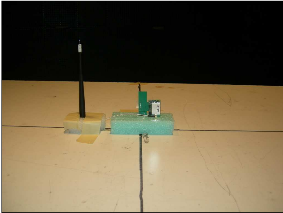
Figure 5: Radiated Emissions Test Setup – ZPOS
