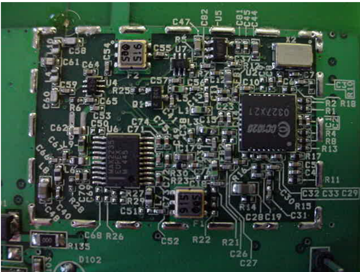
Photo Three – Internal Close Up of RF Section
