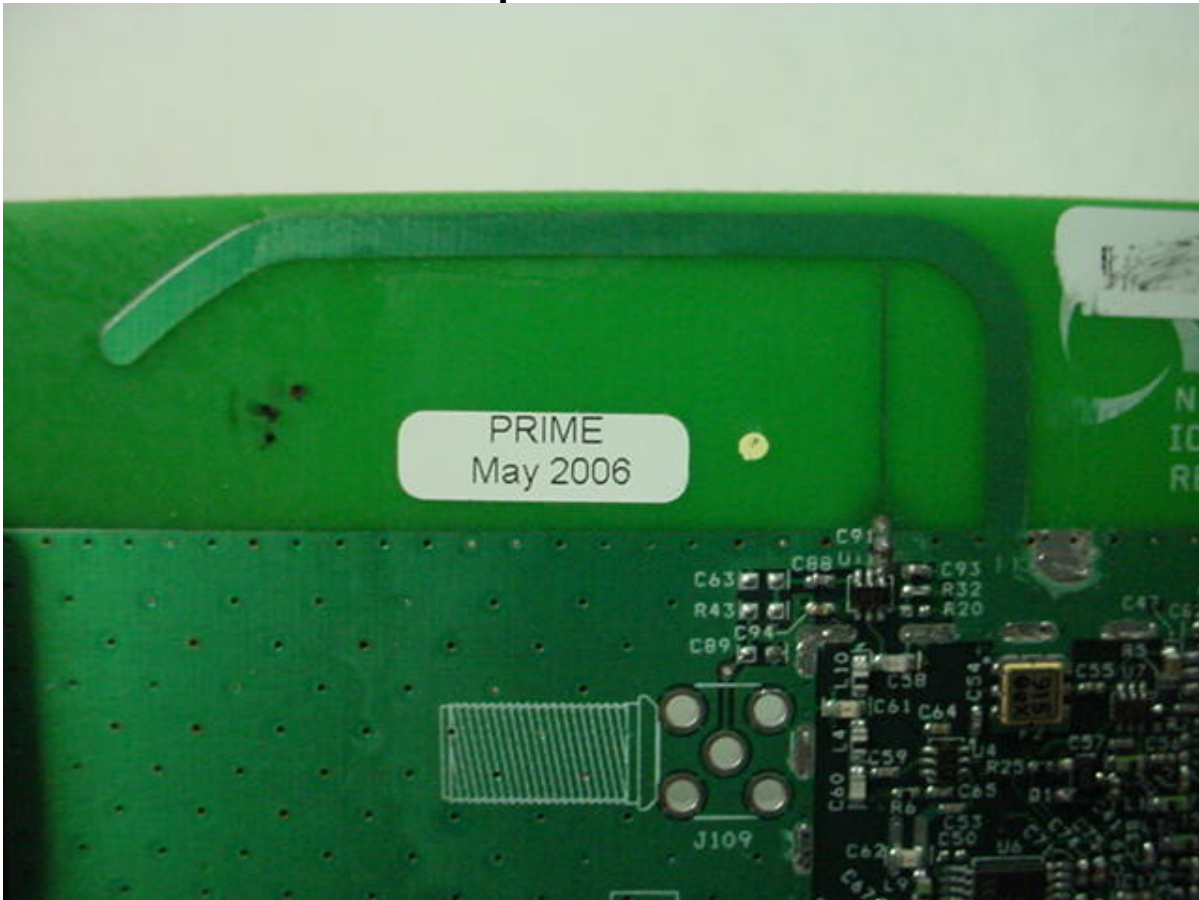
Photo Five – Internal Close up of PCB Antenna
