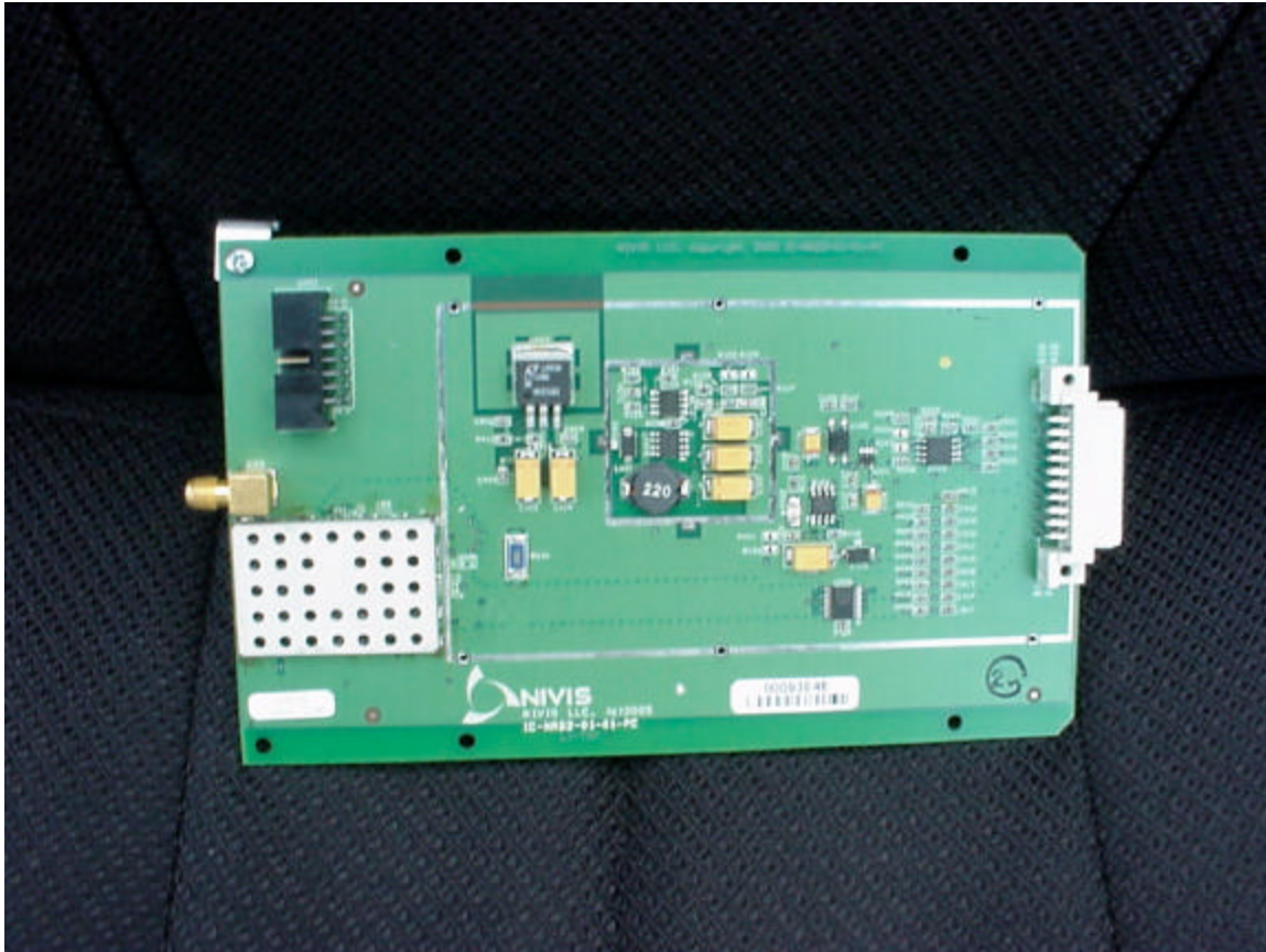
Photo 1. Top View of EUT With Shield in Place
