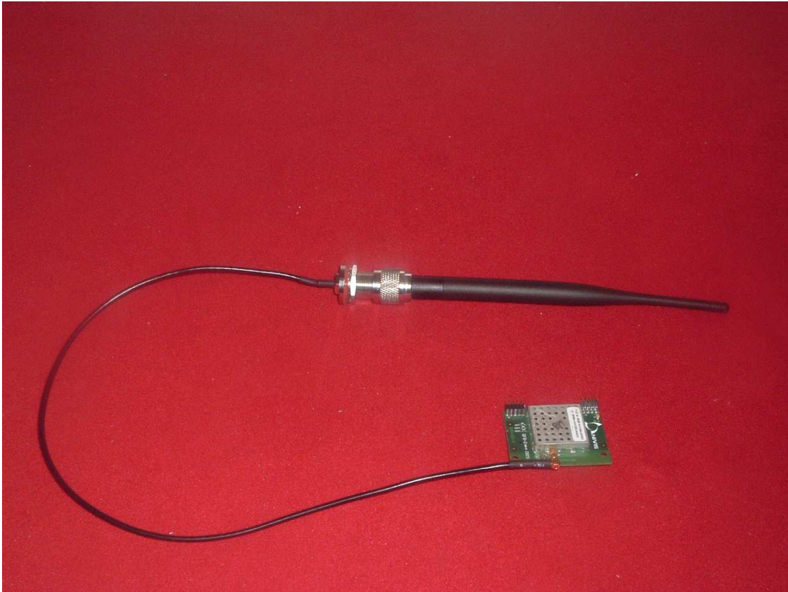
Figure 2: Antenna 1 connected to VN210 Module
