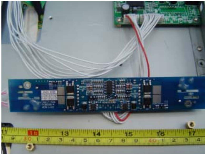
15”&17”Monitor PCB 2 _Internal Photos For Solder View
