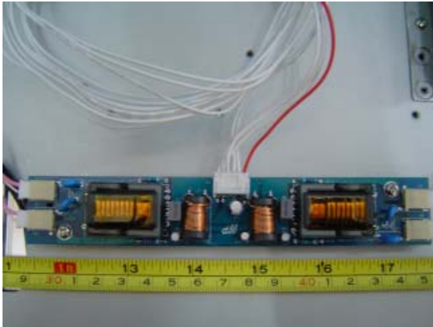
15”&17”Monitor PCB 2 _Internal Photos For Component View
