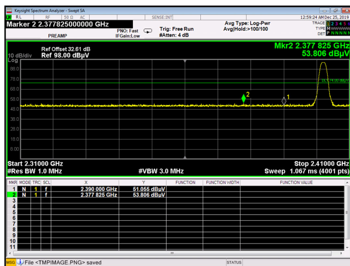
GFSK (1Mbps), LOW CHANNEL, PEAK
