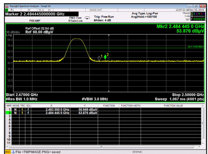
GFSK (1Mbps), HIGH CHANNEL, PEAK
