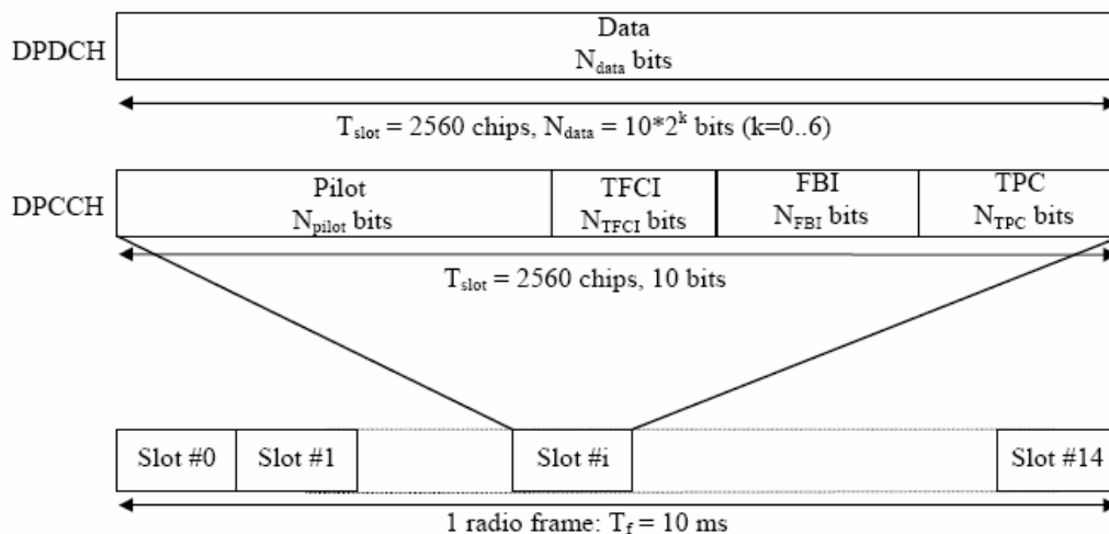
Frame structure for uplink DPDCH/DPCCCH
