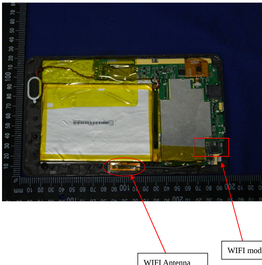
b: Antenna schemes
