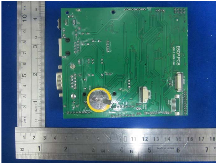
EUT – Sub-Board Board Top View
