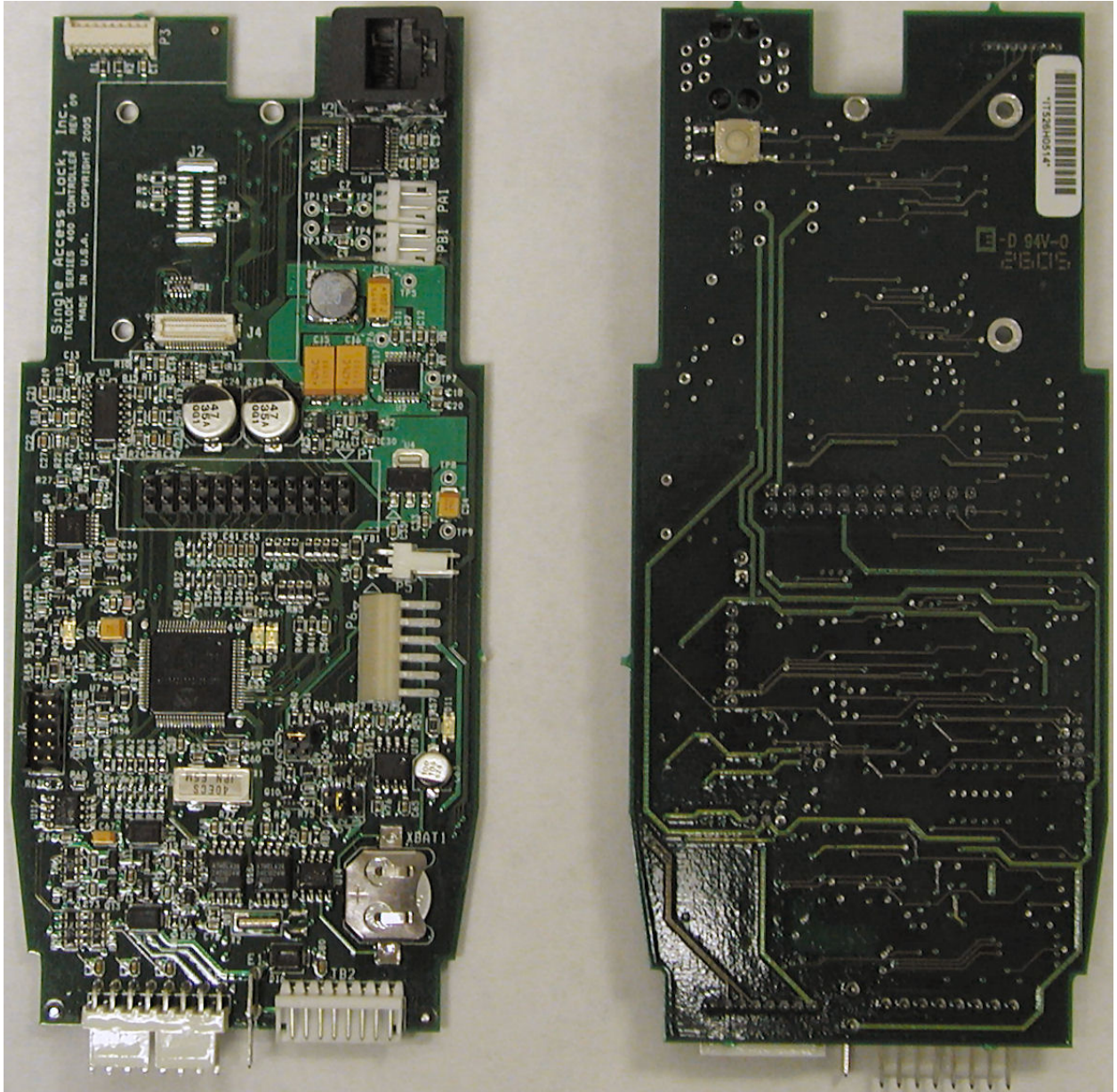
Figure 3: Internal - PCB Front and Back View - Radio Module Removed
