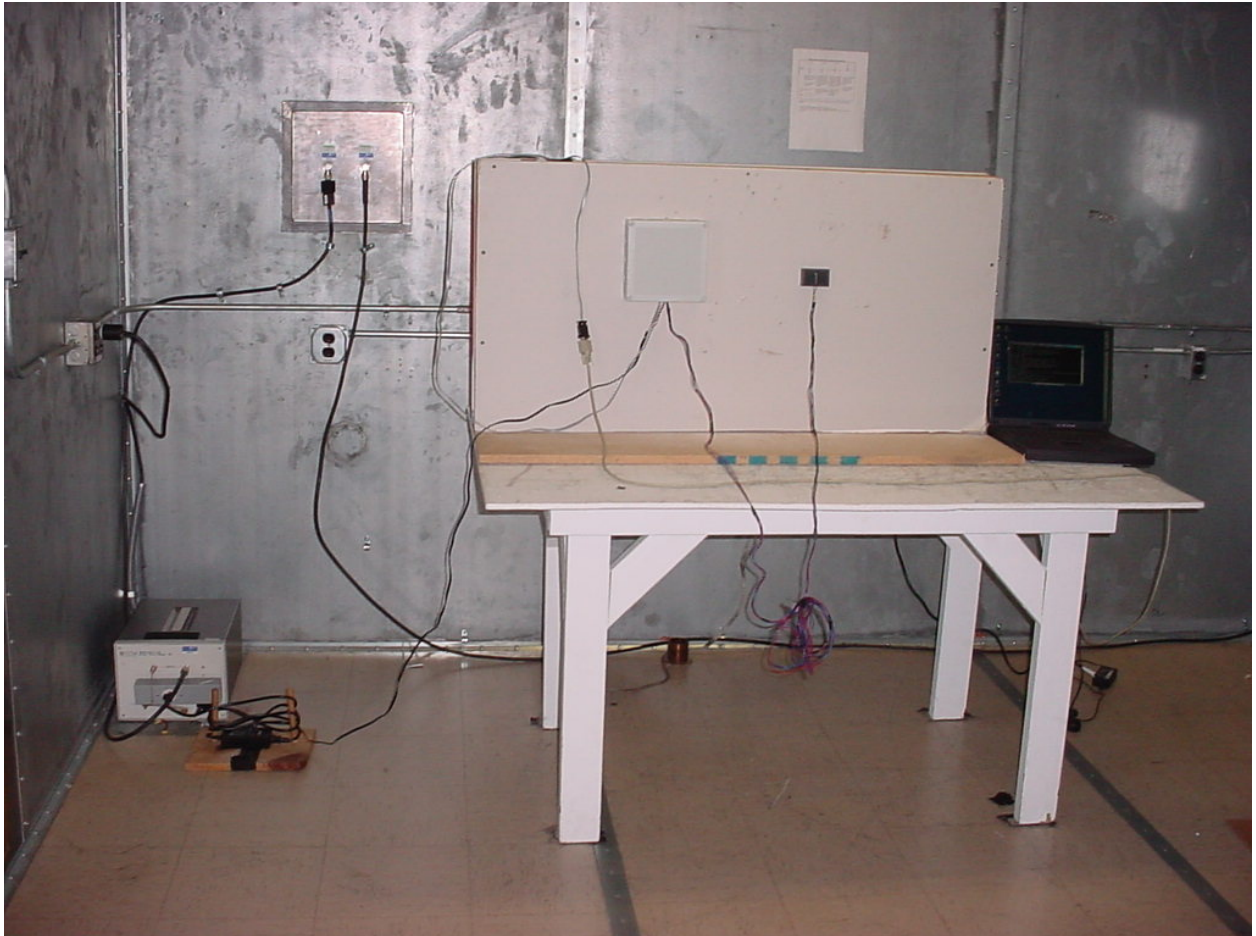
Figure 3: Test Setup – AC Powerline Conducted Emissions – Wall Mount
