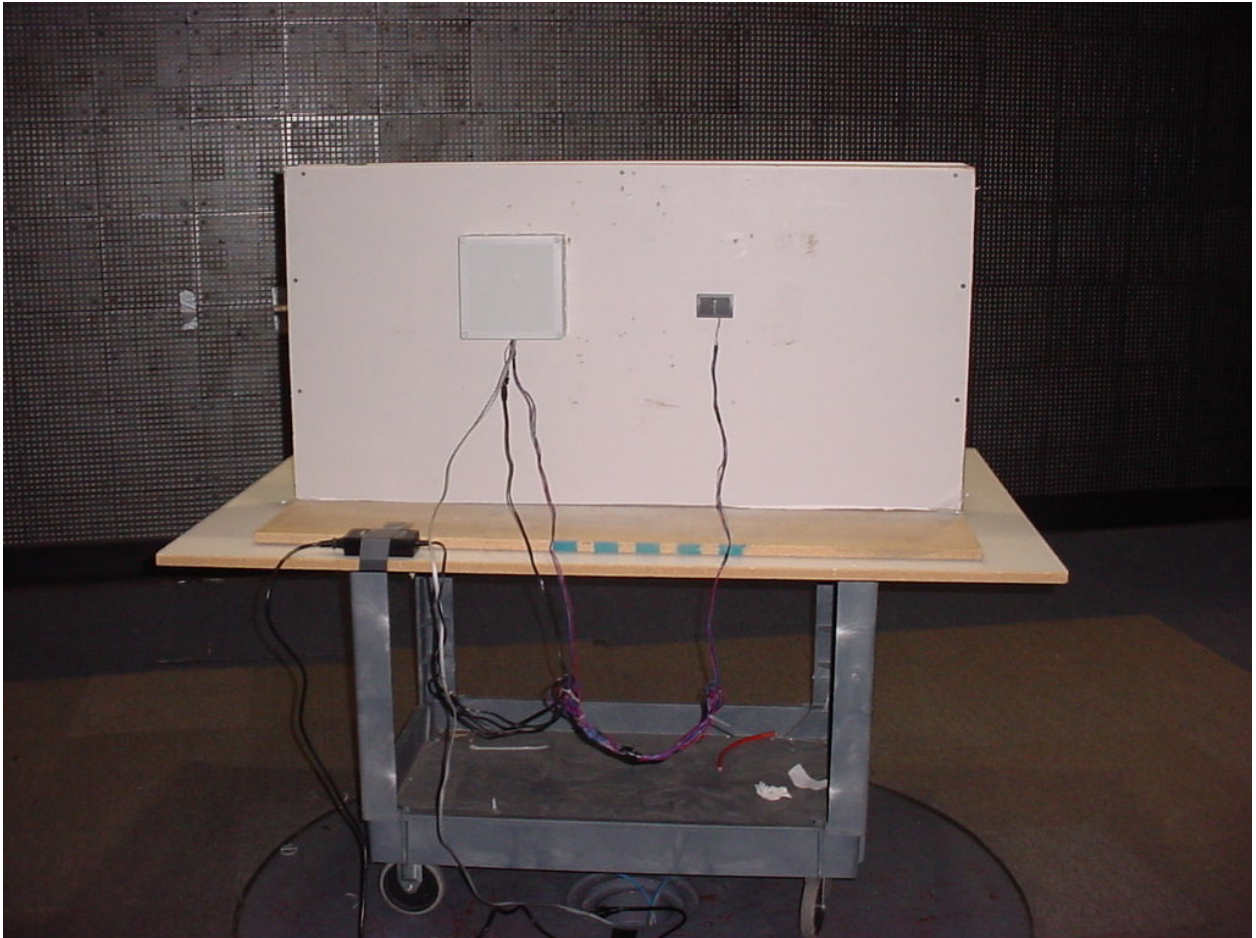
Figure 2: Test Setup – Radiated Emissions – Wall Mount
