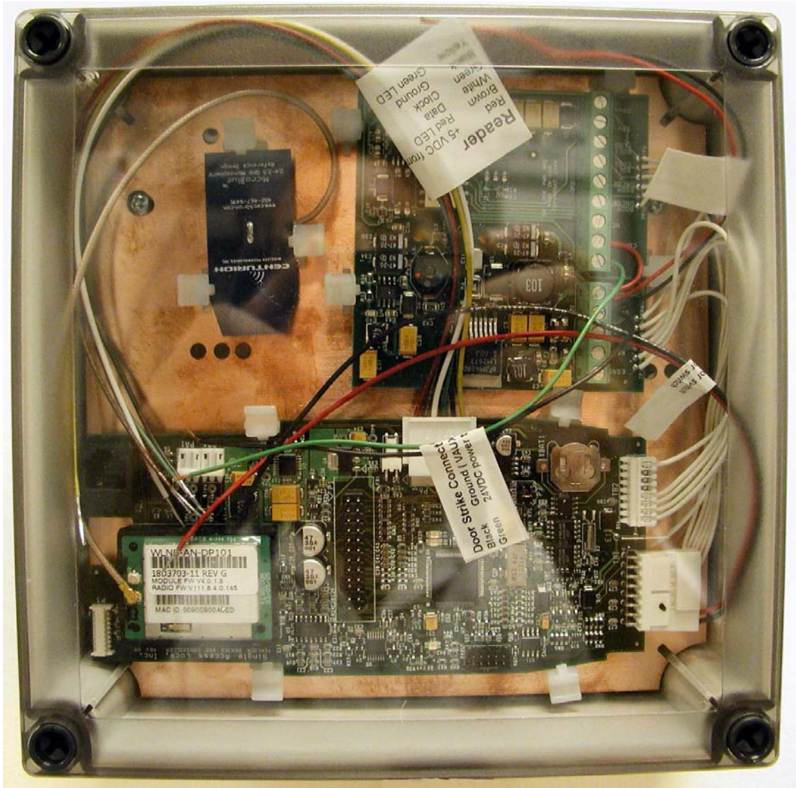
Figure 4: External – Wall Mount Door Controller Front
