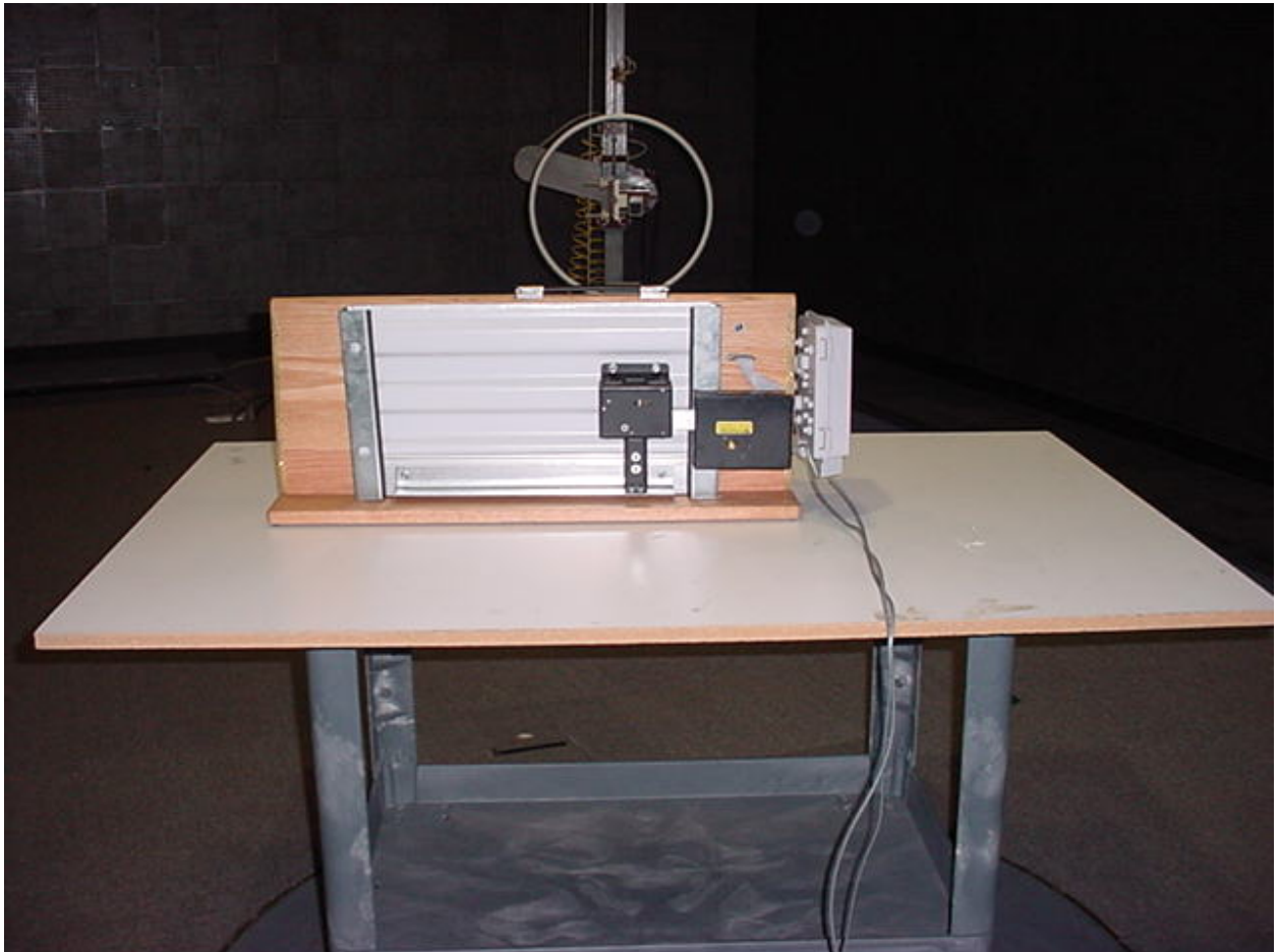
Figure 3: Radiated Emissions – Rollup Door Enclosure (Rear View)
