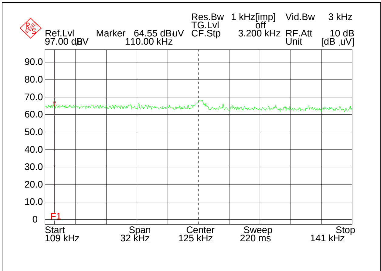
Figure 1. Band-edge Plot
