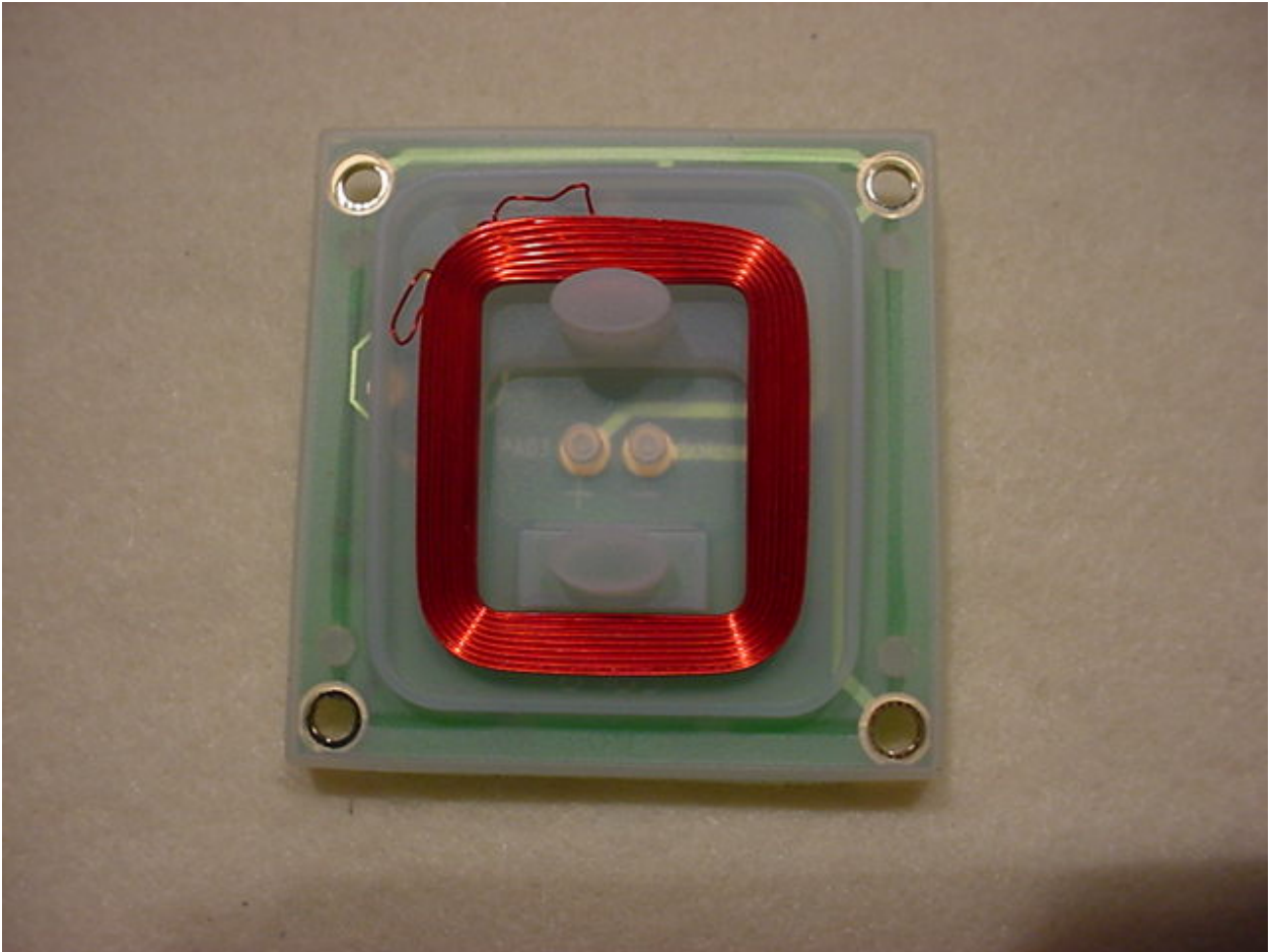
Figure 5: Transmitter Board (Front View - Antenna)
