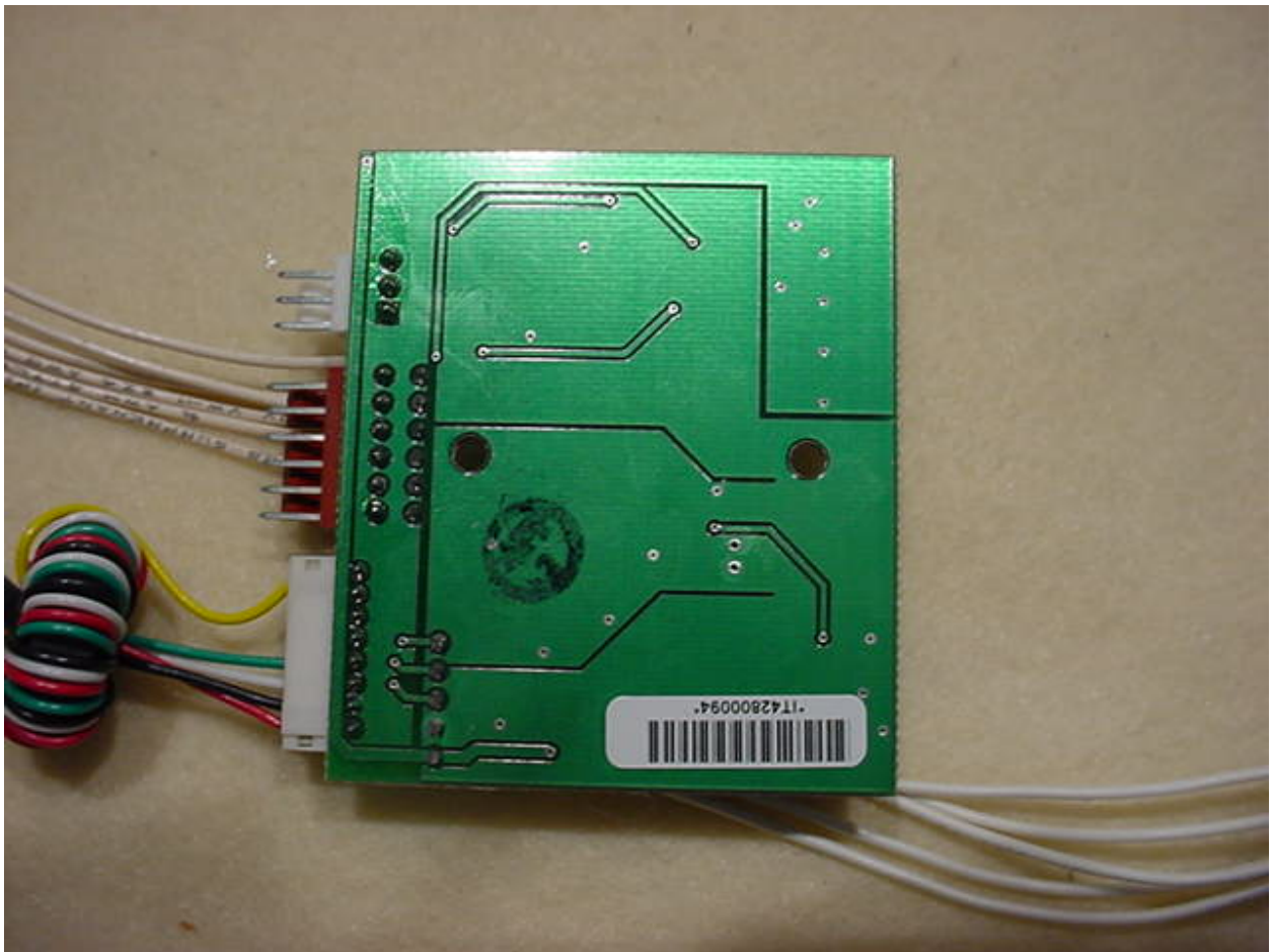
Figure 4: Power Supply Board (Back View)
