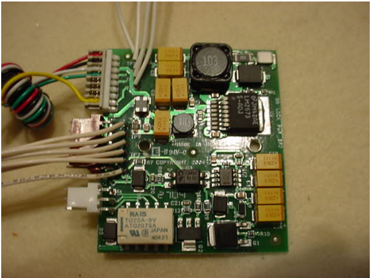
Figure 2: Power Supply Board (Front View)
