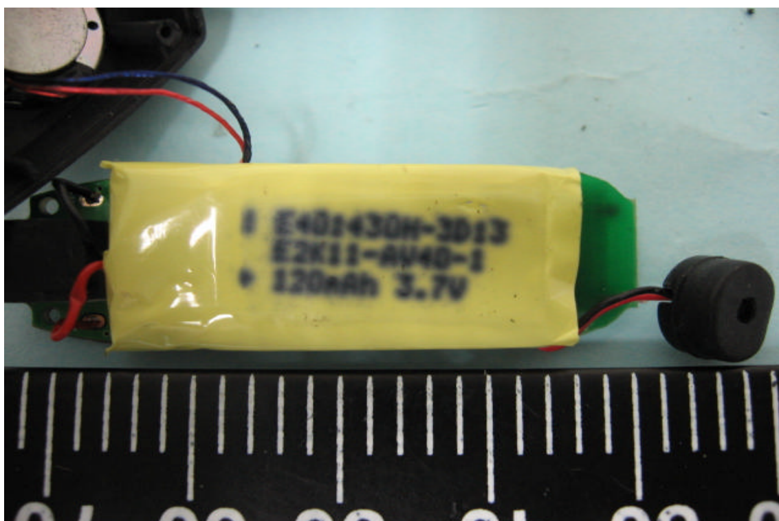
Internal View of EUT (Battery)
