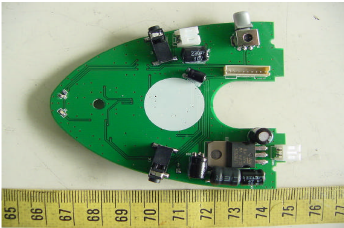
Component View of Car Kit's Main PCB
