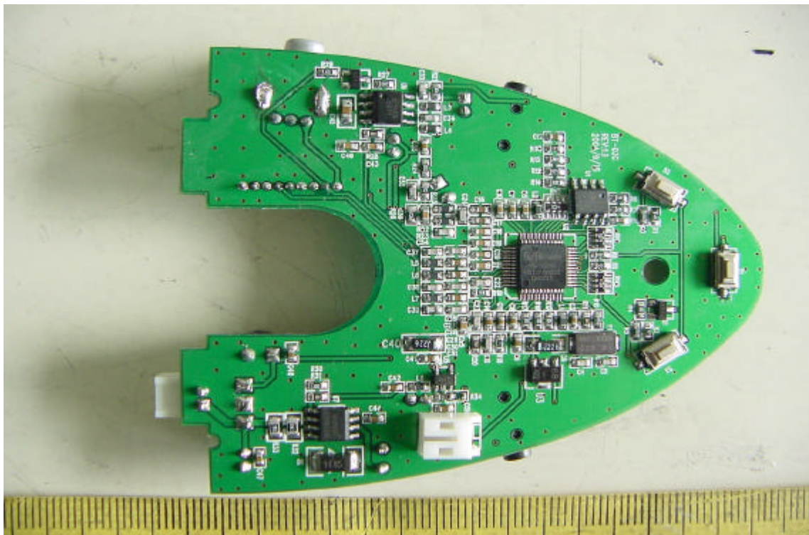
Solder View of Car Kit's Main PCB
