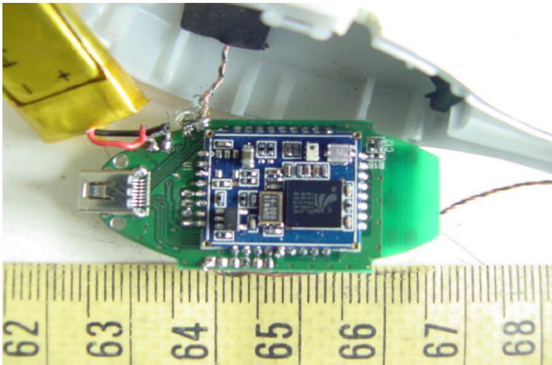
Solder View of Bluetooth Headset's Main PCB
