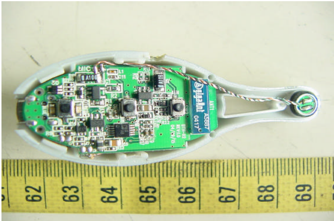
Component View of Bluetooth Headset's Main PCB
