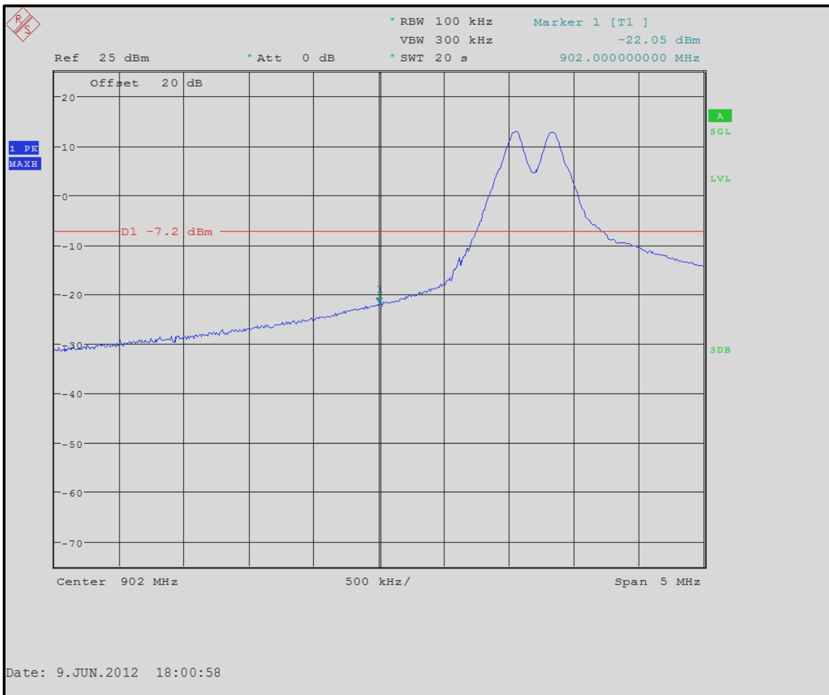
Plot 4-1: Lower Band Edge (902 MHz Band Edge, 903.0 MHz Carrier)
