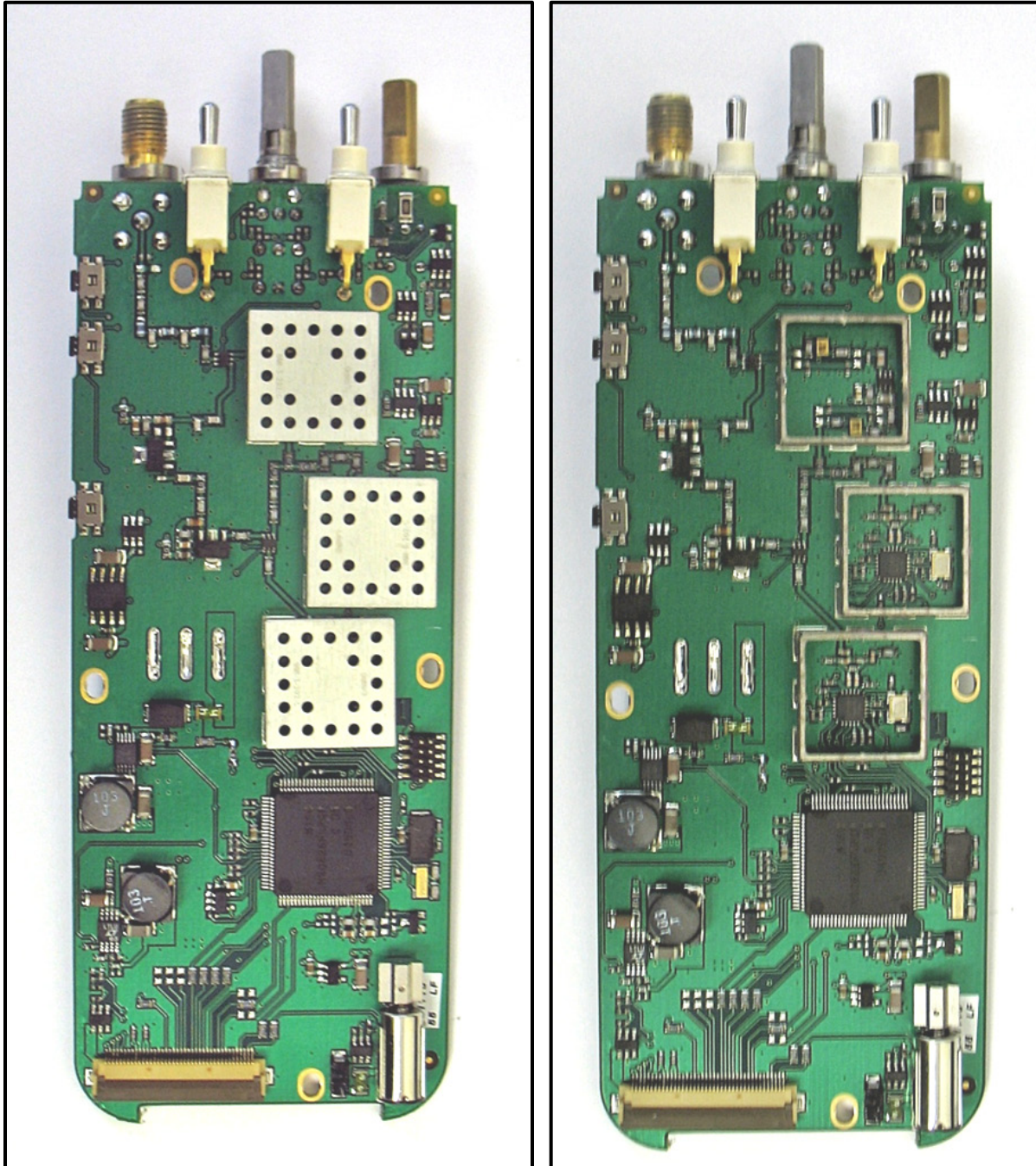
Photograph 2: Radio Board with Shields and Radio Board without Shields
