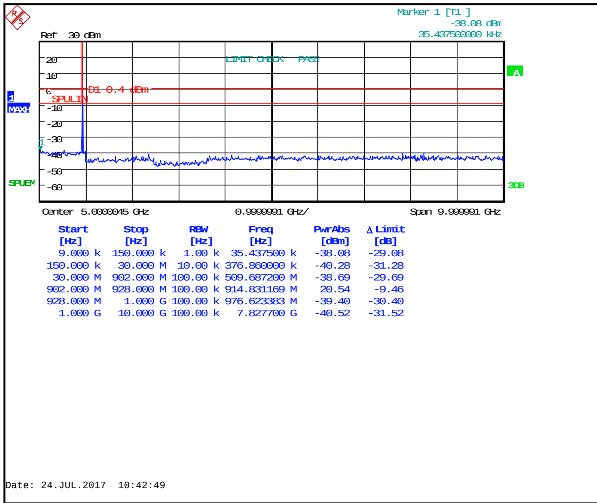
Plot 5-2: Antenna Conducted Spurious Emissions (914.980 MHz)
