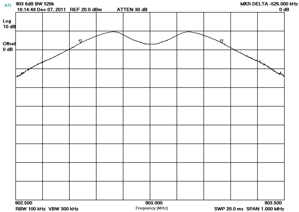
Plot 6-1: 6 dB Bandwidth; 903 MHz; 526 kHz
