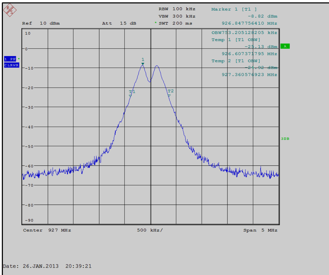
Plot 6-3: 6 dB Bandwidth – 927.0 MHz
