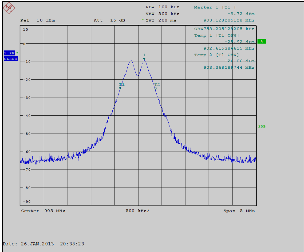
Plot 6-1: 6 dB Bandwidth – 903.0 MHz
