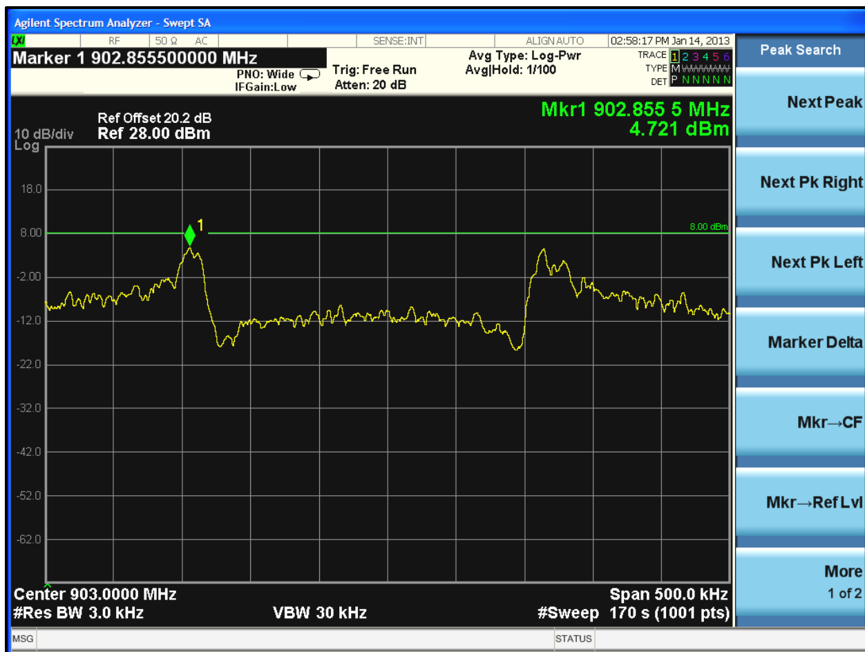
Plot 7-1: Power Spectral Density – 903.0 MHz
