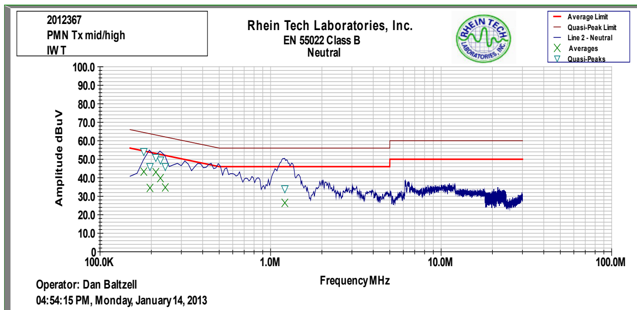
Plot 8-4: Conducted Emissions (Neutral Side); Mode: Transmit Yagi Antenna
