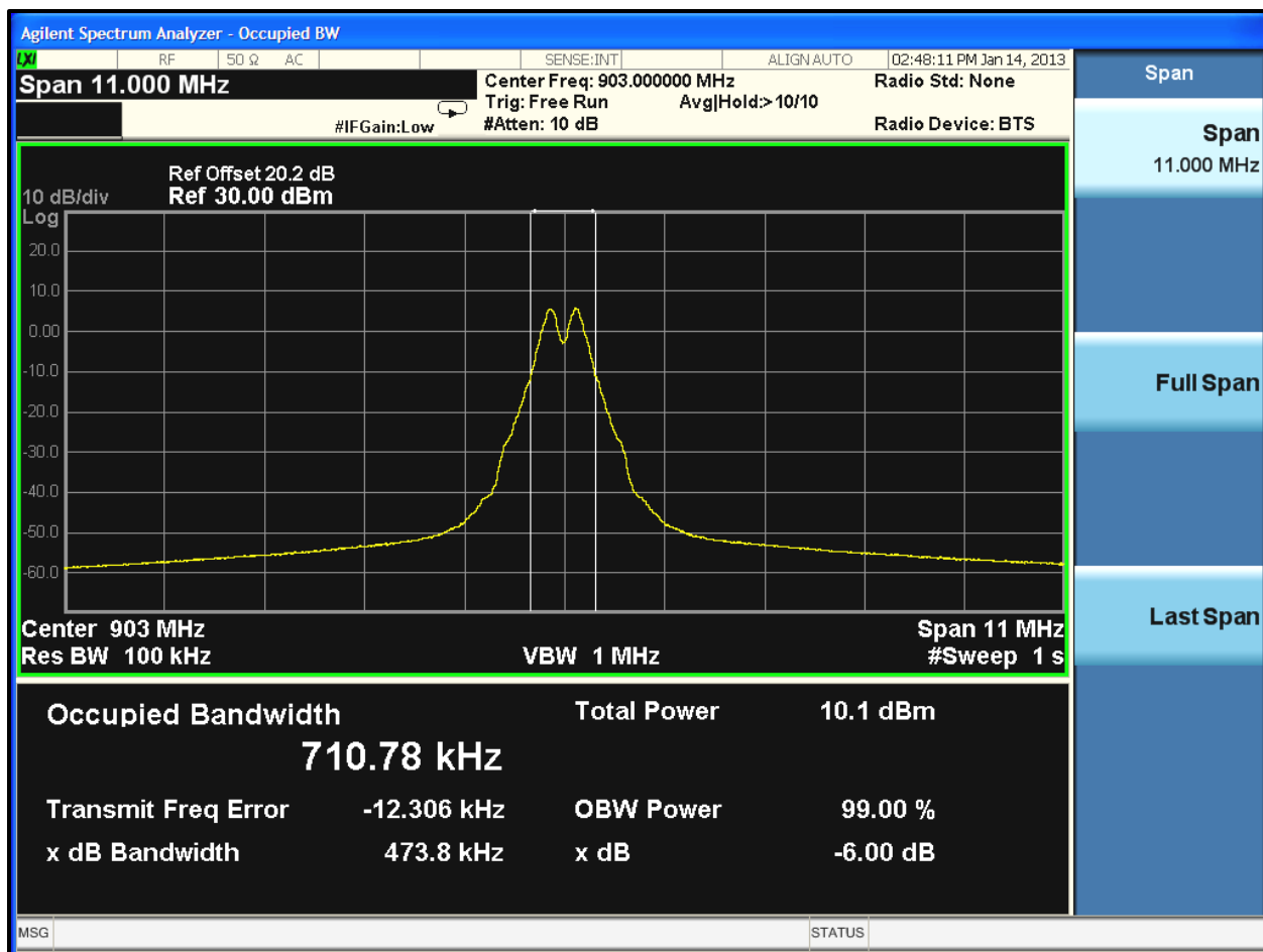
Plot 6-1: 6 dB Bandwidth – 903.0 MHz
