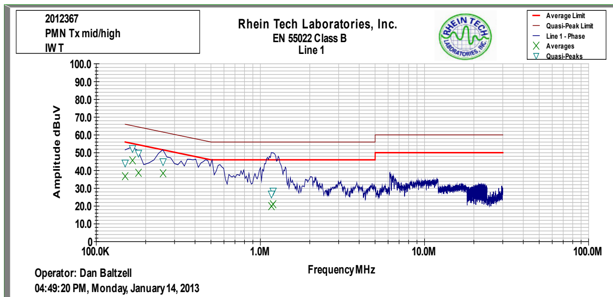
Plot 8-3: Conducted Emissions (Phase Side); Mode: Transmit Yagi Antenna
